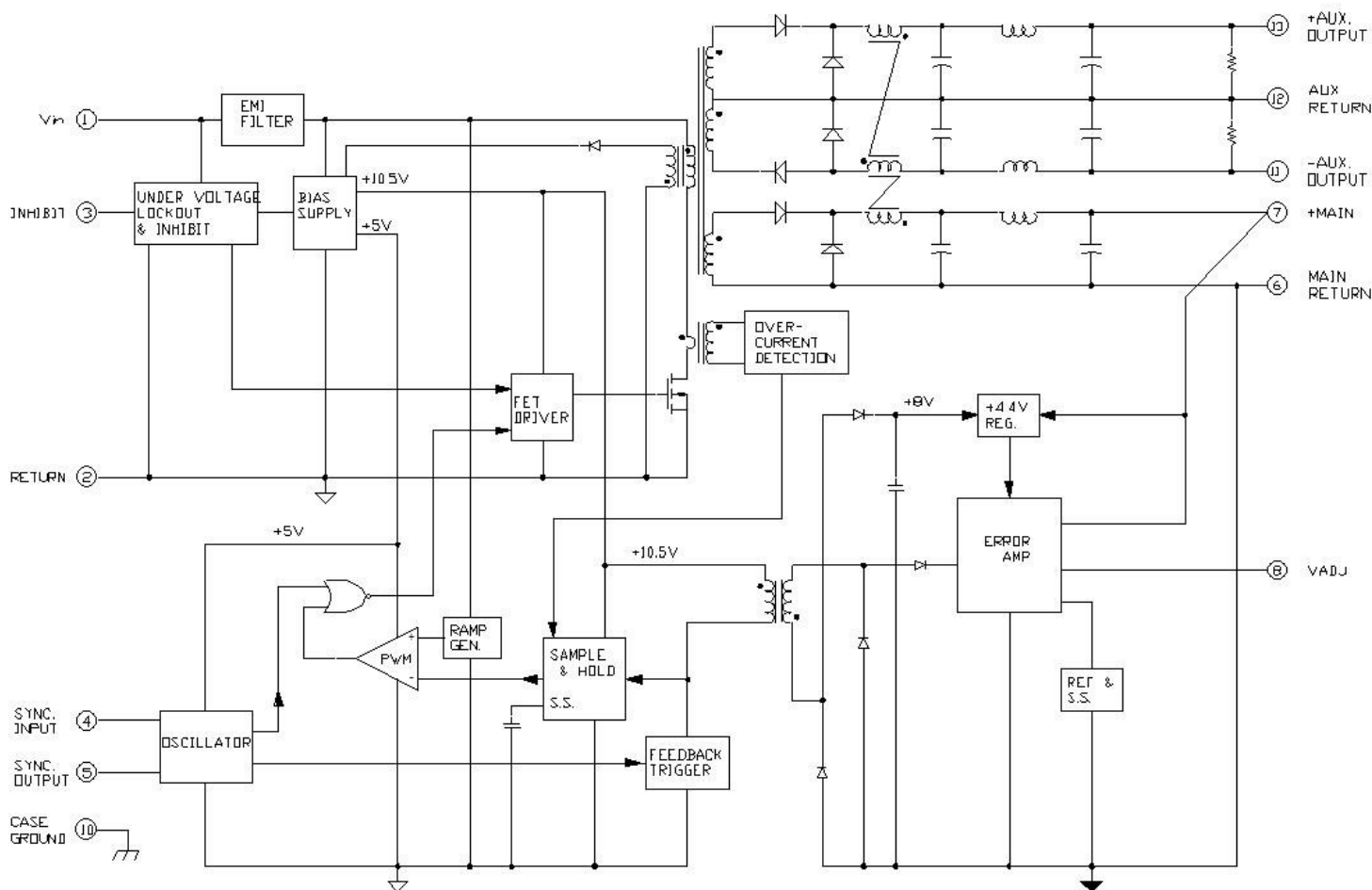
Fig 1. Block Diagram
