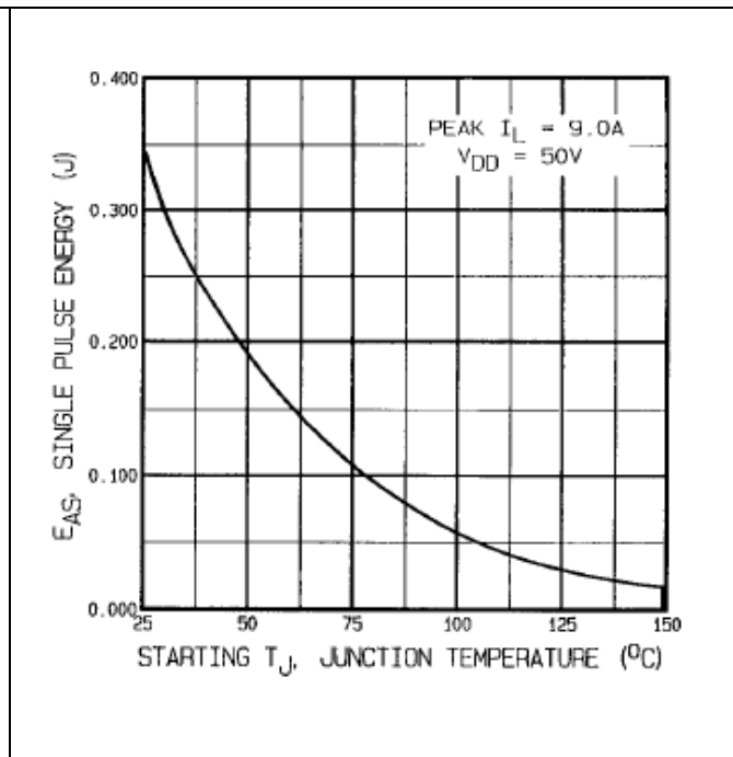
Figure 11 Maximum Avalanche Energy Vs. Junction Temperature
