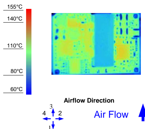
Figure 8. Thermal Image for Airflow Direction 3 (6A output, 55°C ambient, 200 LFM, typical Vin, open frame, unit soldered onto a fixture board)
