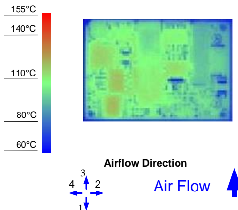
Figure 8. Thermal Image for Airflow Direction 3 (3A output, 55°C ambient, 0 LFM, typical Vin, open frame, unit soldered onto a fixture board)
