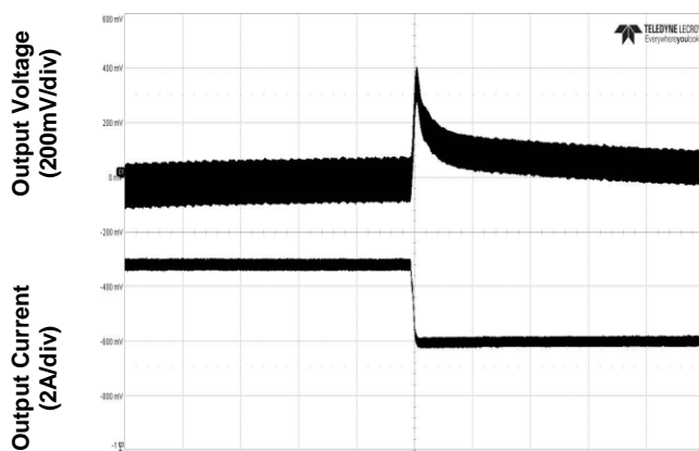
Figure 5. Transient Load Response (typical Vin, load current steps from 75% to 50% at a slew rate 0.1A/µs)
