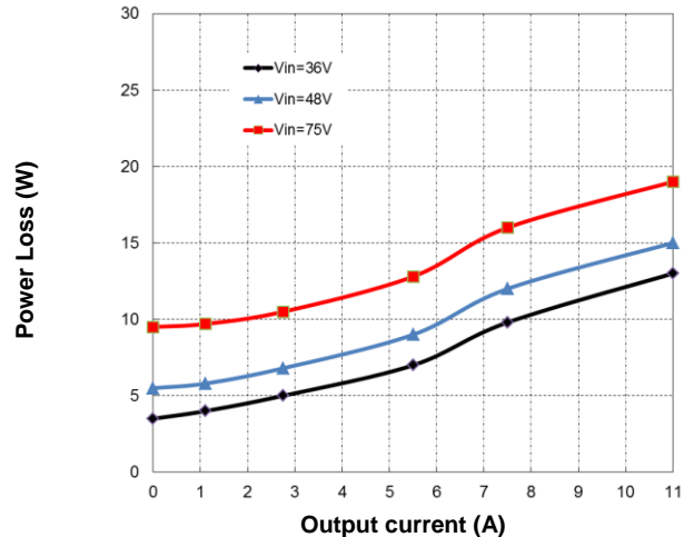
Figure 2. output Characteristic (25°C)
