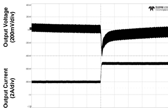
Figure 6. Transient Load Response (typical Vin, load current steps from 50% to 75% at a slew rate 0.1A/µs)
