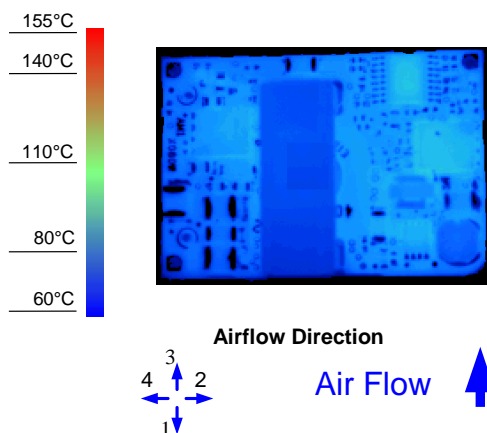
Figure 8. Thermal Image for Airflow Direction 3 (7A output, 55°C ambient, 200 LFM, typical Vin, open frame, unit soldered onto a fixture board)
