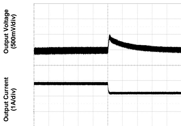
Time – t (500μs/div) Figure 5. Transient Load Response (typical Vin, load current steps from 75% to 50% at a slew rate 0.1A/μs)
