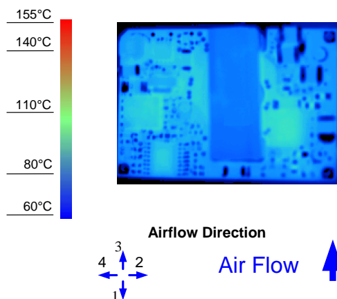
Figure 8. Thermal Image for Airflow Direction 3 (2.5A output, 55°C ambient, 200 LFM, typical Vin, open frame, unit soldered onto a fixture board)
