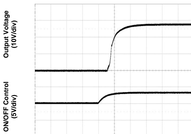
Time – t (10ms/div) Figure 4. Start-Up from Enable Control (typical Vin, full load)
