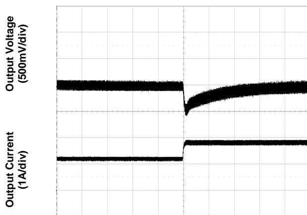
Time – t (500μs/div) Figure 6. Transient Load Response (typical Vin, load current steps from 50% to 75% at a slew rate 0.1A/μs)
