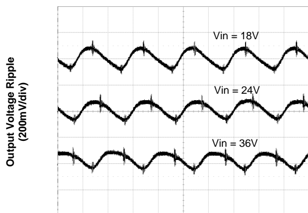
Time – t (20μs/div) Figure 3. Output Ripple Voltage at Full Load
