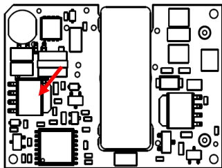
Figure 15. Temperature Monitoring Locations
