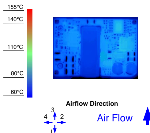
Figure 8. Thermal Image for Airflow Direction 3 (4A output, 55°C ambient, 200 LFM, Vin=36V, open frame, unit soldered onto a fixture board)
