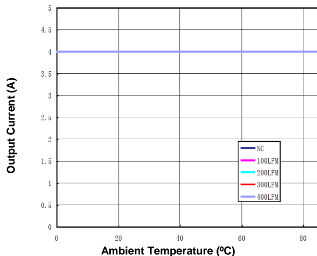
Figure 7. Current Derating Curve with Open Frame (Direction 3 (Ref. Figure 8); Vin=36V, unit soldered onto a fixture board)
