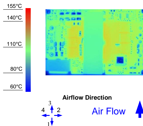
Figure 8. Thermal Image for Airflow Direction 3 (8A output, 85°C ambient, 200 LFM, typical Vin, open frame, soldered interface)
