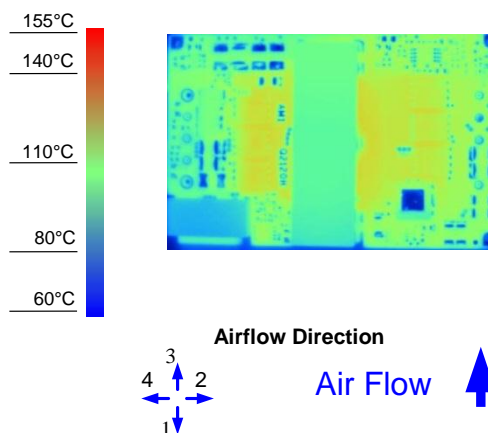
Figure 8. Thermal Image for Airflow Direction 3 (10A output, 55°C ambient, 200 LFM, typical Vin, open frame, soldered interface)
