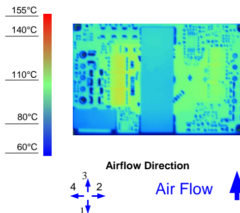
Figure 8. Thermal Image for Airflow Direction 3 (19A output, 55°C ambient, 200 LFM, typical Vin, open frame, soldered interface)
