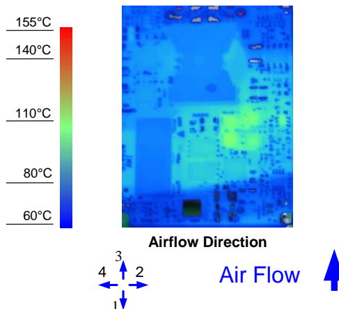
Figure 8. Thermal Image for Airflow Direction 3 (2A output, 55°C ambient, 200 LFM, typical Vin, open frame, unit soldered onto a fixture board)
