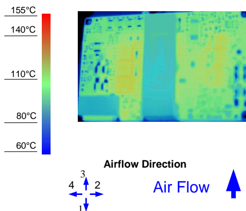
Figure 8. Thermal Image for Airflow Direction 3 (25A output, 55°C ambient, 200 LFM, typical Vin, open frame, soldered interface)
