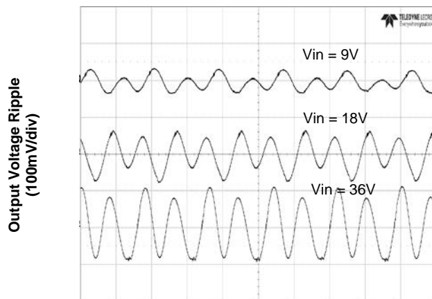
Figure 4. Output Ripple Voltage at Full Load
