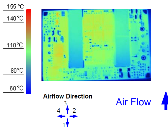
Figure 8. Thermal Image for Airflow Direction 3 (31.5A output, 55°C ambient, 200 LFM, typical Vin, open frame, soldered interface)
