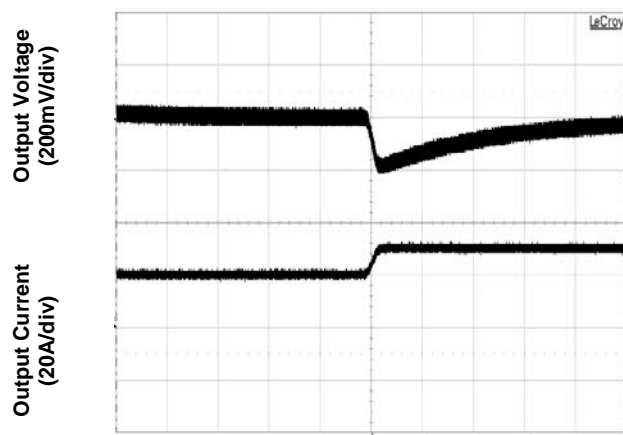
Figure 5. Transient Load Response (typical V_{in} , load current steps from 50% to 75% at a slew rate 0.1A/ \mu s)
