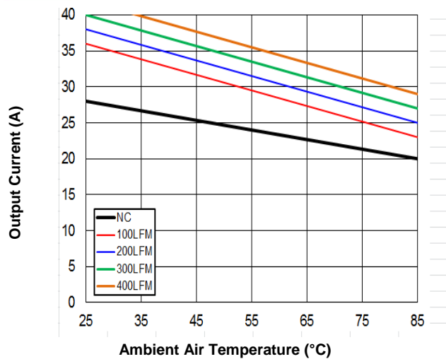
Figure 7. Current Derating Curve for Airflow Direction 3 (Ref. Fig. 8 for Airflow Direction; typical Vin, open frame, unit soldered onto a fixture board)
