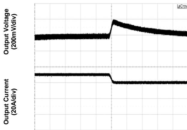
Figure 6. Transient Load Response (typical V_{in} , load current steps from 75% to 50% at a slew rate 0.1A/ \mu s)
