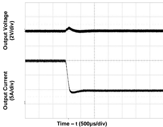
Figure 7. Transient Load Response (typical Vin, load current steps from 14A to 5A at a slew rate 0.1A/µs)
