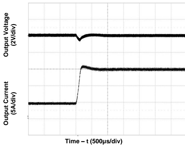
Figure 8. Transient Load Response (typical Vin, load current steps from 5A to 14A at a slew rate 0.1A/µs)
