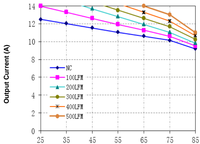
Figure 9. Current Derating Curve for Airflow Direction 3 (Ref. Fig. 10 for Airflow Direction; typical Vin, open frame)
