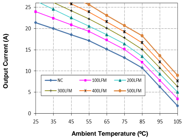
Figure 13a. Derating with Open-frame ( V_{in}=24V and V_o=3.3V )
