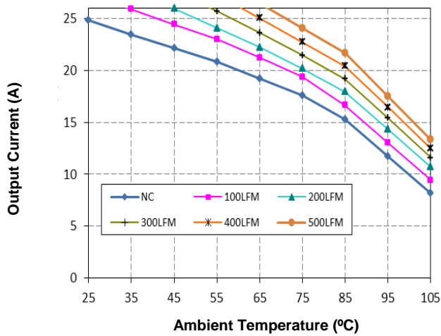
Figure 12a. Derating with Open-frame ( V_{in}=12V and V_o=3.3V )
