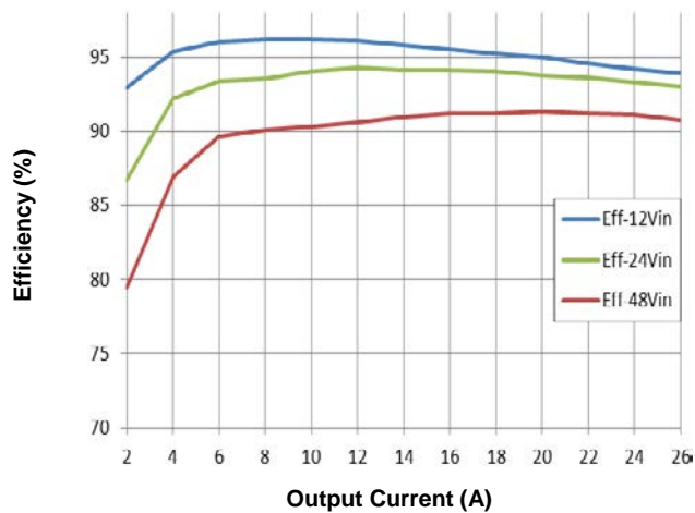
Figure 8. Efficiency Vs. Load Current (Vo=5V)
