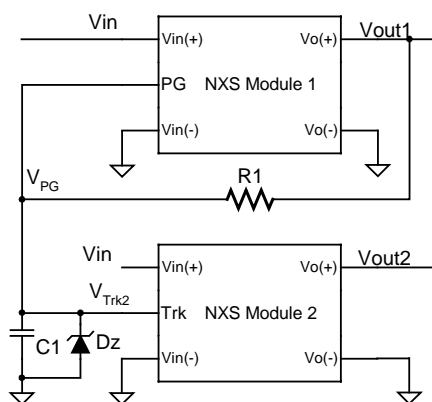
Figure 26. Circuit Configuration for Sequential Startup
