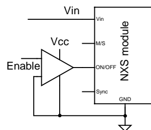
Figure 20. Direct Logic Drive
