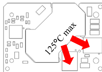
Figure 29. Thermal Monitoring Points
