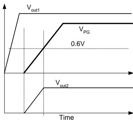
Figure 27. Sequential Startup Waveforms
