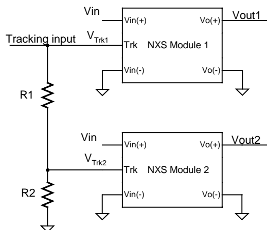
Figure 24. Circuit Configuration for Simultaneous Tracking
