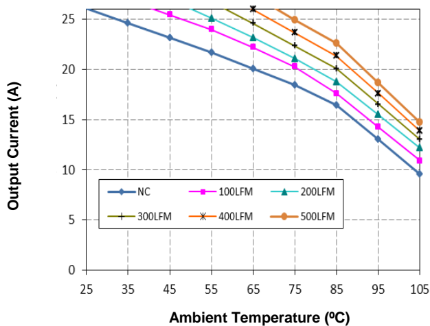
Figure 14a. Derating with Open-frame ( V_{in}=12V and V_o=5V )
