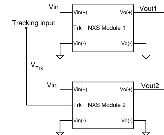
Figure 22. Circuit Configuration for Ratio-metric Tracking
