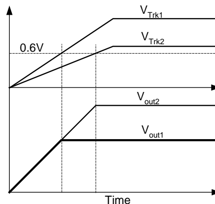
Figure 25. Simultaneous Tracking Waveforms
