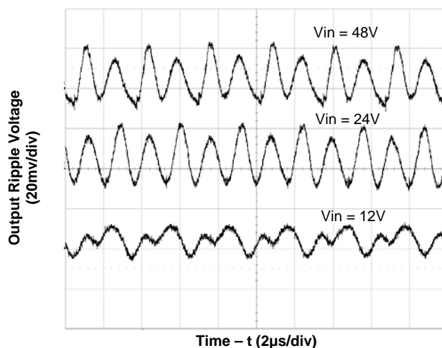
Figure 2. Output Ripple Voltage ( V_o=5V ; I_o=20A ; C_{o,ex}=470\mu F )
