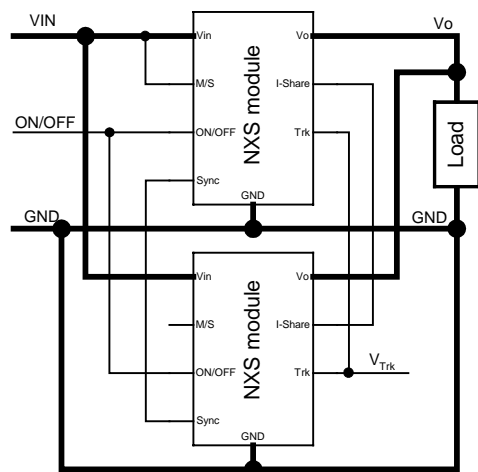
Figure 28. Circuit Configuration for Active Load Sharing
