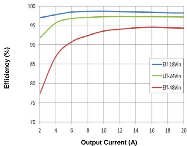
Figure 11. Efficiency Vs. Load Current (Vo=15V)
