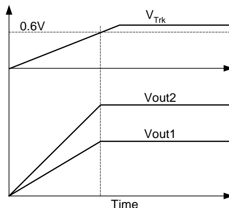
Figure 23. Ratio-metric Tracking Waveforms
