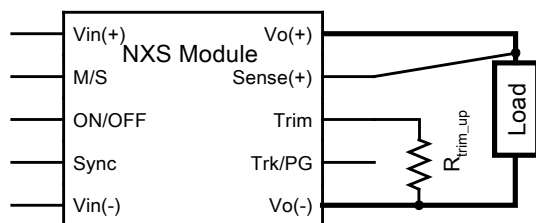
Figure 21. Circuit Configuration for Output Voltage Trim Up
