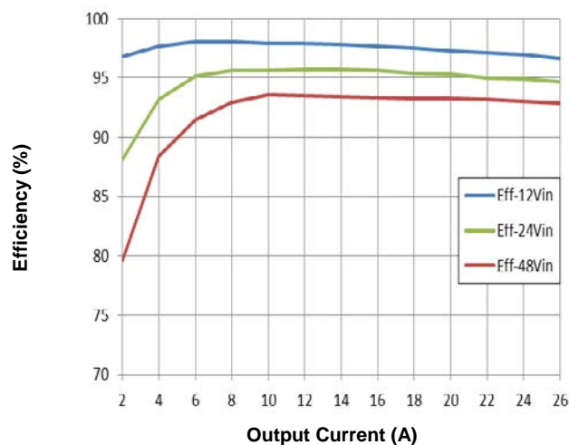
Figure 9. Efficiency Vs. Load Current (Vo=9V)
