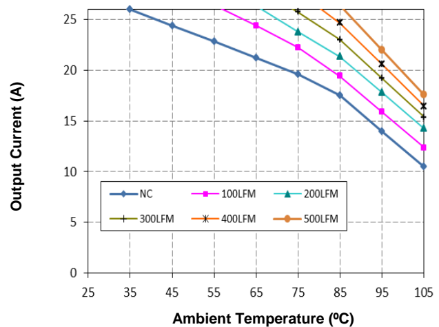
Figure 14b. Derating with Baseplate ( V_{in}=12V and V_o=5V )
