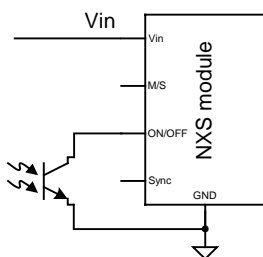
Figure 18. Opto-coupler Enable Circuit
