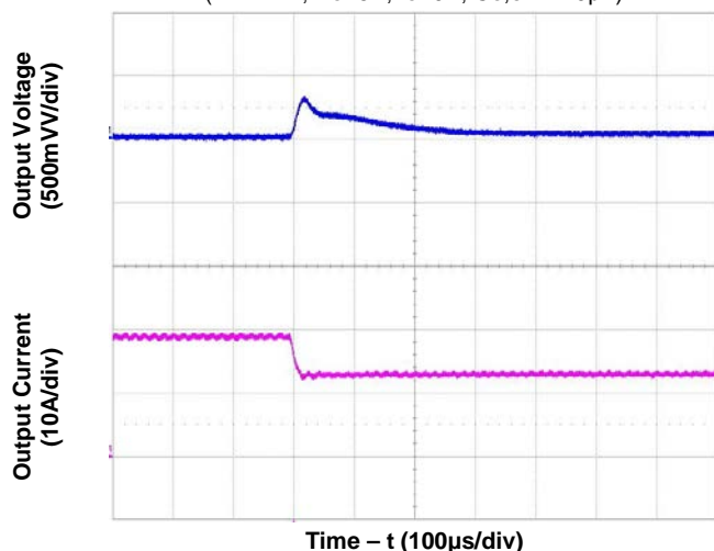
Figure 3. Transient Load Response at V_o=5V ( V_{in}=12V ; I_o=19.5A \rightarrow 13A @ 0.1A/\mu s ; C_{o,ex}=470\mu F )
