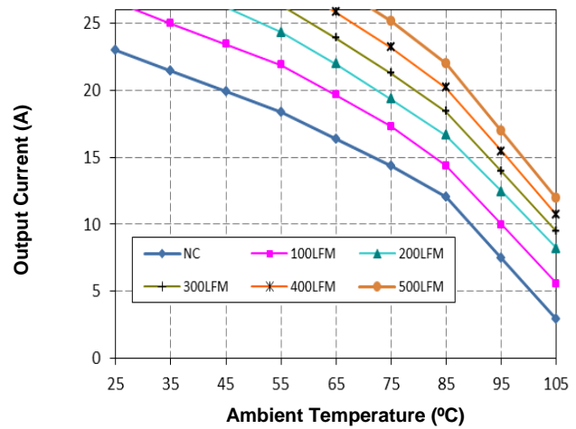
Figure 13b. Derating with Baseplate ( V_{in}=24V and V_o=3.3V )
