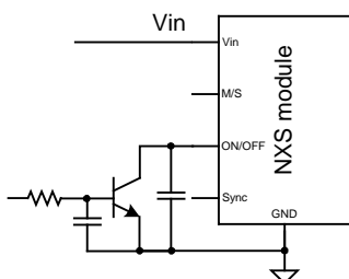
Figure 19. Open Collector Enable Circuit
