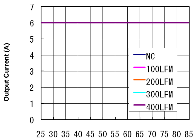
Ambient Temperature (°C) Figure 8d. Current Derating Curve (Vin=12V, Vo=2.5V, open frame)
