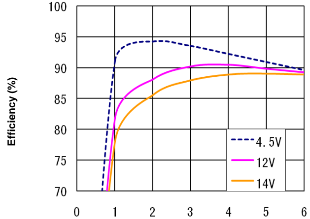
Figure 1d. Efficiency vs. Load Current (25°C, V_o=2.5V )
