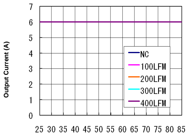
Ambient Temperature (°C) Figure 8c. Current Derating Curve (Vin=12V, Vo=1.5V, open frame)
