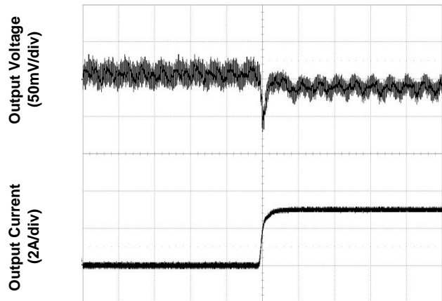
Figure 3. Transient Load Response (typical V_{in} , V_o=5V , load current steps from 0% to 50% at a slew rate 1A/ \mu s)
