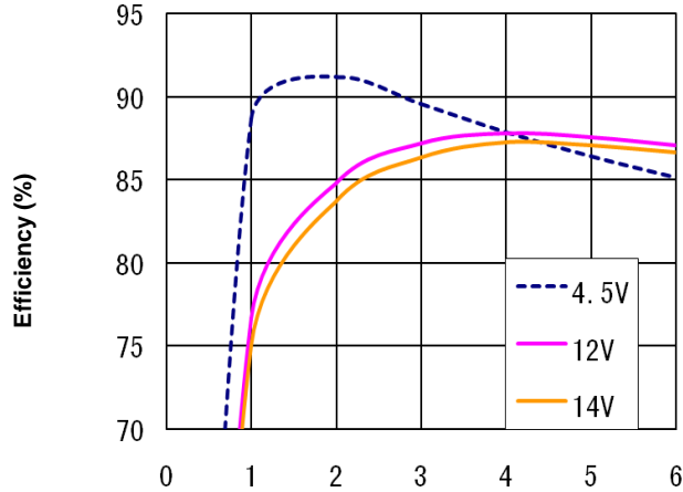
Figure 1c. Efficiency vs. Load Current (25°C, V_o=1.8V )
