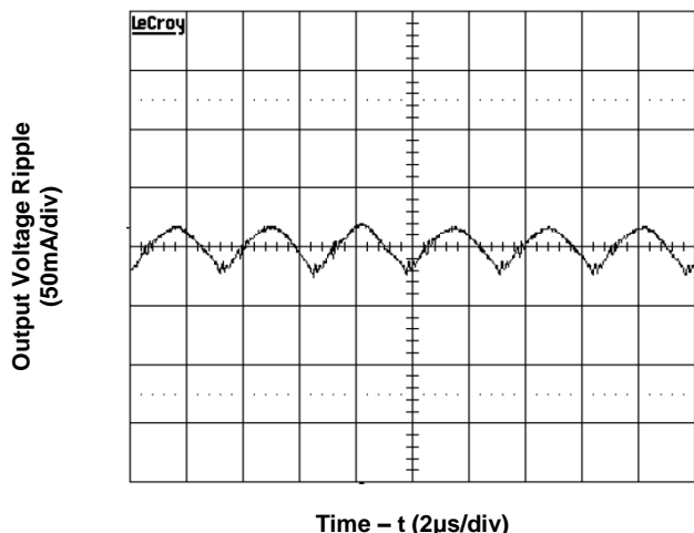
Figure 4c. Output Voltage Ripple (Vin=12V, full load)
