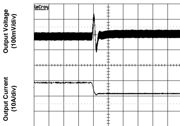
Figure 6f. Transient Load Response (typical Vin, load current steps from 75% to 50% at a slew rate 0.1A/µs)
