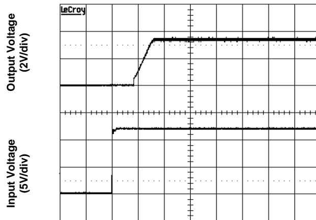
Figure 5d. Output Voltage (Vin=12V, full load)
