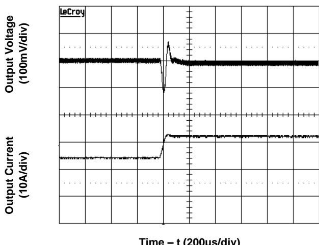
Figure 3e. Transient Load Response (typical Vin, load current steps from 50% to 75% at a slew rate 0.1A/µs)
