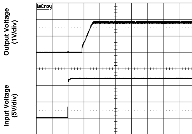
Figure 3d. Output Voltage (Vin=12V, full load)
