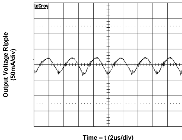
Figure 5c. Output Voltage Ripple (Vin=12V, full load)
