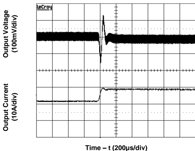
Figure 6e. Transient Load Response (typical Vin, load current steps from 50% to 75% at a slew rate 0.1A/µs)
