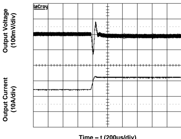
Figure 4e. Transient Load Response (typical Vin, load current steps from 50% to 75% at a slew rate 0.1A/µs)
