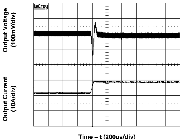
Figure 5e. Transient Load Response (typical Vin, load current steps from 50% to 75% at a slew rate 0.1A/µs)
