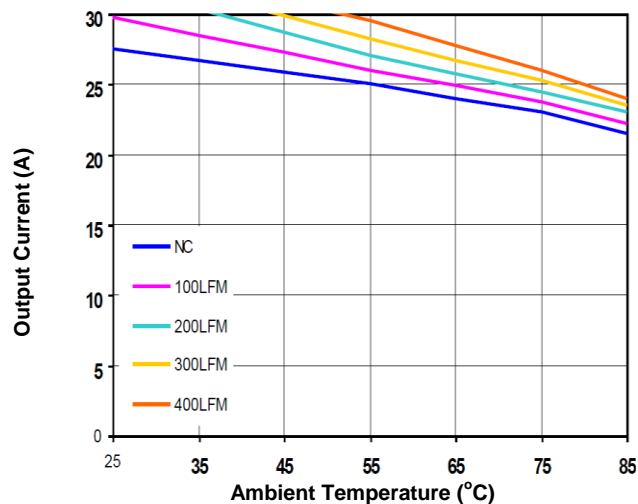
Figure 3b. Current Derating Curve (Vin=12V, open frame)
