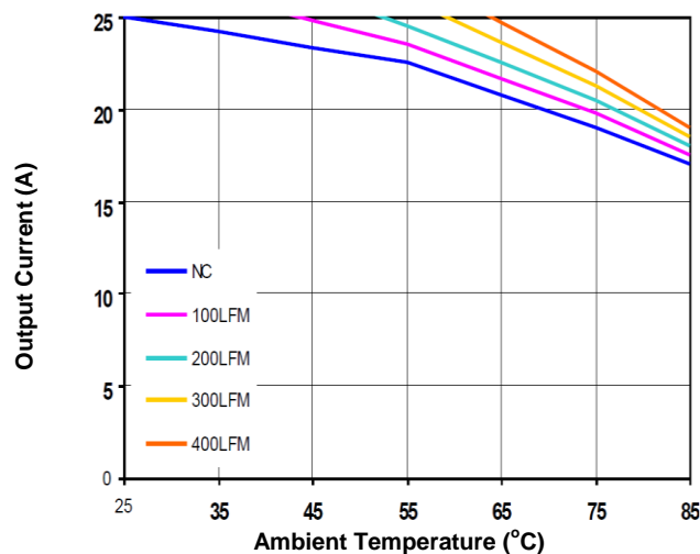
Figure 5b. Current Derating Curve (Vin=12V, open frame)
