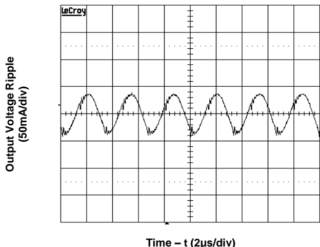
Figure 6c. Output Voltage Ripple (Vin=12V, full load)
