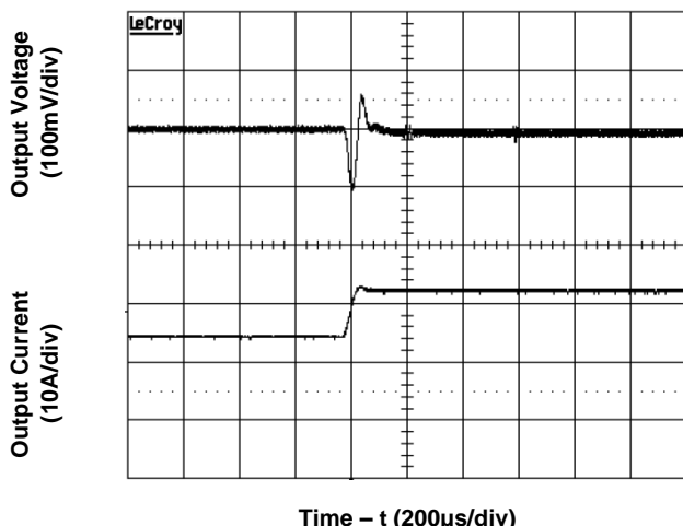
Figure 2e. Transient Load Response (typical Vin, load current steps from 50% to 75% at a slew rate 0.1A/µs)
