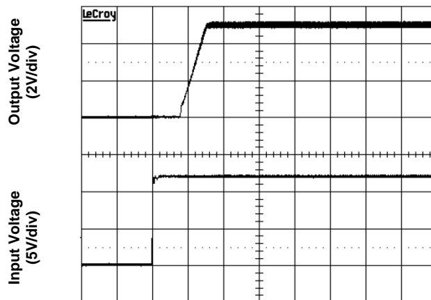
Figure 6d. Output Voltage (Vin=12V, full load)
