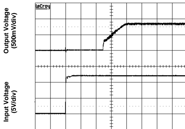
Figure 1d. Output Voltage (Vin=12V, full load)
