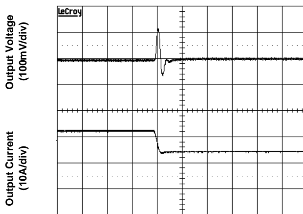
Figure 1f. Transient Load Response (typical Vin, load current steps from 75% to 50% at a slew rate 0.1A/µs)
