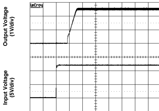
Figure 4d. Output Voltage (Vin=12V, full load)
