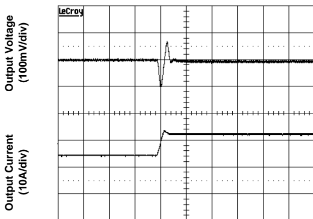
Figure 1e. Transient Load Response (typical Vin, load current steps from 50% to 75% at a slew rate 0.1A/µs)
