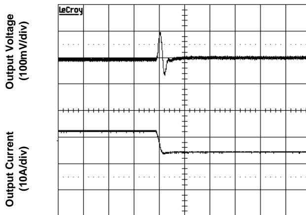
Figure 2f. Transient Load Response (typical Vin, load current steps from 75% to 50% at a slew rate 0.1A/µs)
