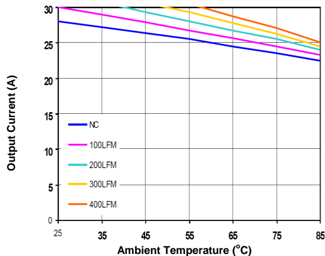
Figure 2b. Current Derating Curve (Vin=12V, open frame)
