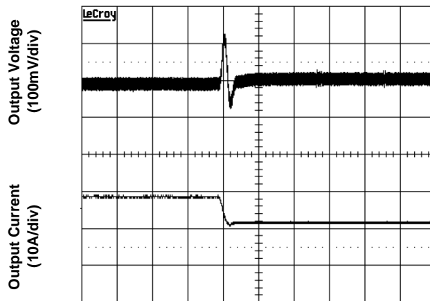
Figure 5f. Transient Load Response (typical Vin, load current steps from 75% to 50% at a slew rate 0.1A/µs)
