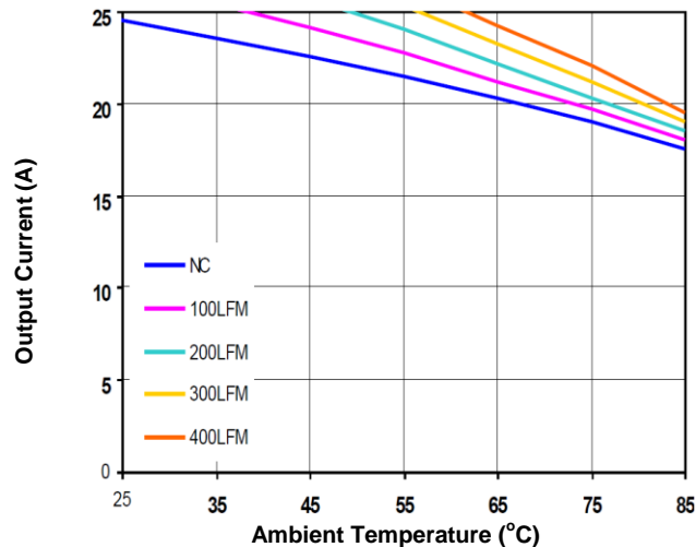
Figure 6b. Current Derating Curve (Vin=12V, open frame)
