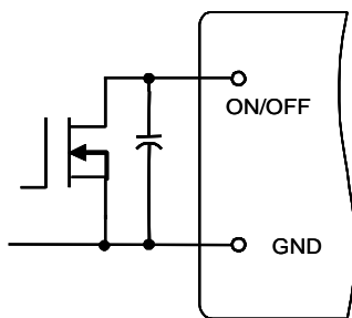
Figure 7. Circuit for Positive Logic Control
