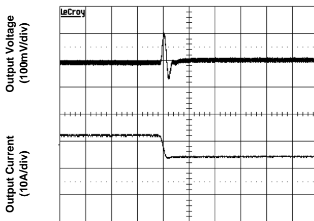
Figure 3f. Transient Load Response (typical Vin, load current steps from 75% to 50% at a slew rate 0.1A/µs)
