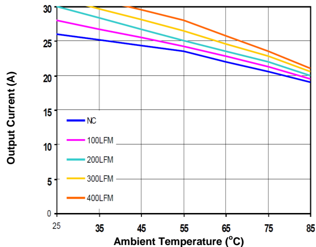
Figure 4b. Current Derating Curve (Vin=12V, open frame)
