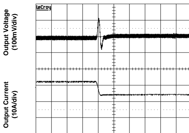
Figure 4f. Transient Load Response (typical Vin, load current steps from 75% to 50% at a slew rate 0.1A/µs)
