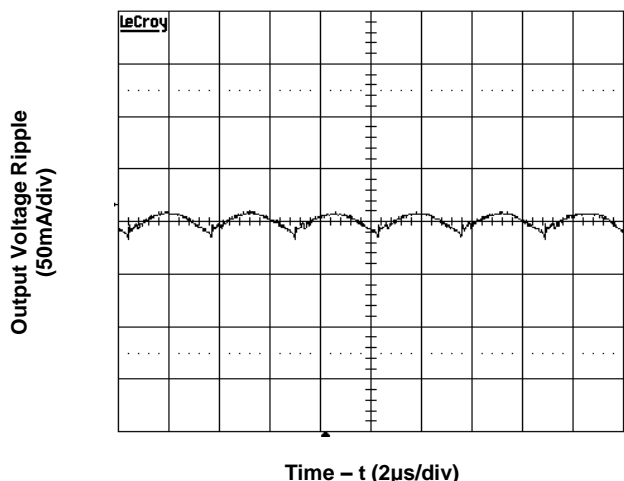
Figure 2c. Output Voltage Ripple (Vin=12V, full load)
