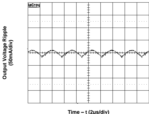
Figure 3c. Output Voltage Ripple (Vin=12V, full load)
