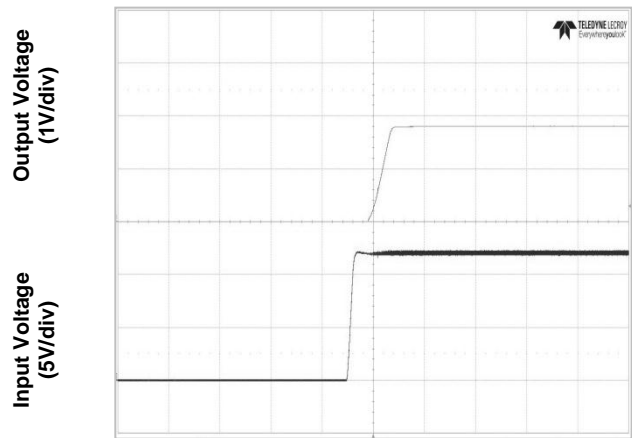
Figure 3d. Start-Up from Application of Input Voltage (Vin=12V, full load)
