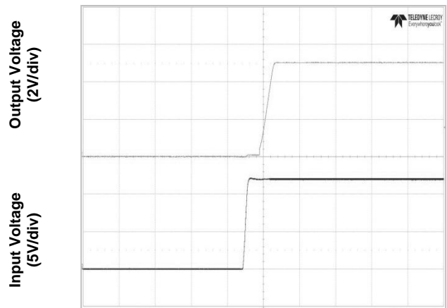
Figure 6d. Start-Up from Application of Input Voltage (Vin=12V, full load)
