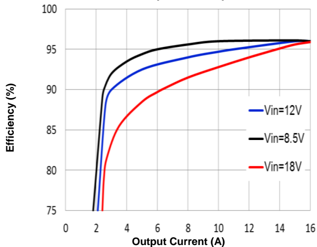
Figure 5a. Efficiency vs. Load Current (25°C)
