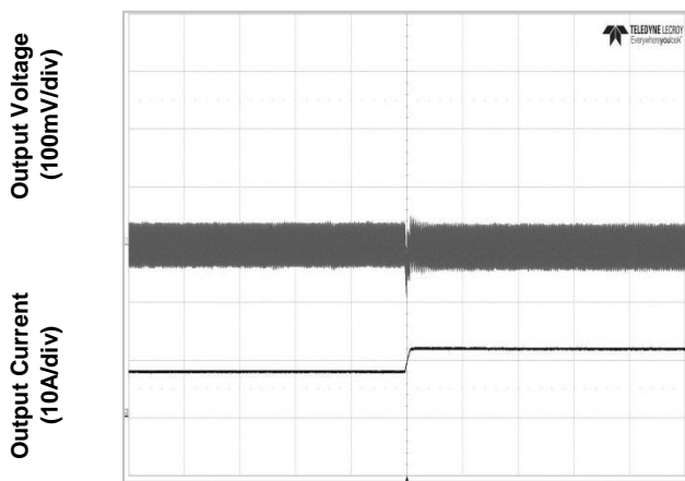
Figure 4e. Transient Load Response (typical Vin, load current steps from 50% to 75% at a slew rate 0.1A/µs)
