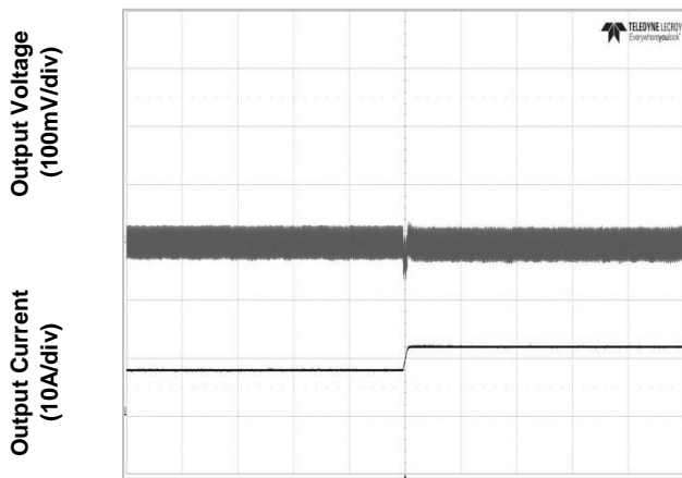
Figure 3e. Transient Load Response (typical Vin, load current steps from 50% to 75% at a slew rate 0.1A/µs)
