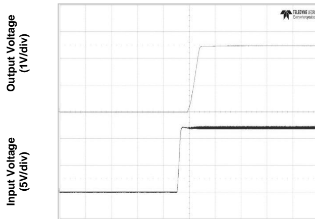
Figure 4d. Start-Up from Application of Input Voltage (Vin=12V, full load)
