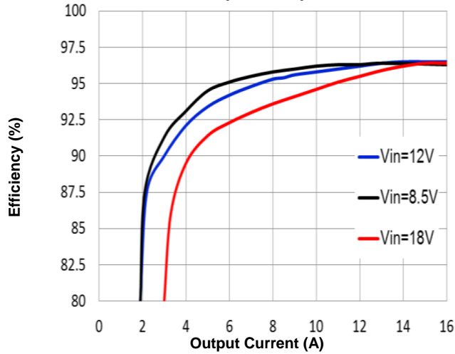
Figure 6a. Efficiency vs. Load Current (25°C)
