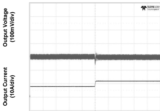
Figure 2e. Transient Load Response (typical Vin, load current steps from 50% to 75% at a slew rate 0.1A/µs)
