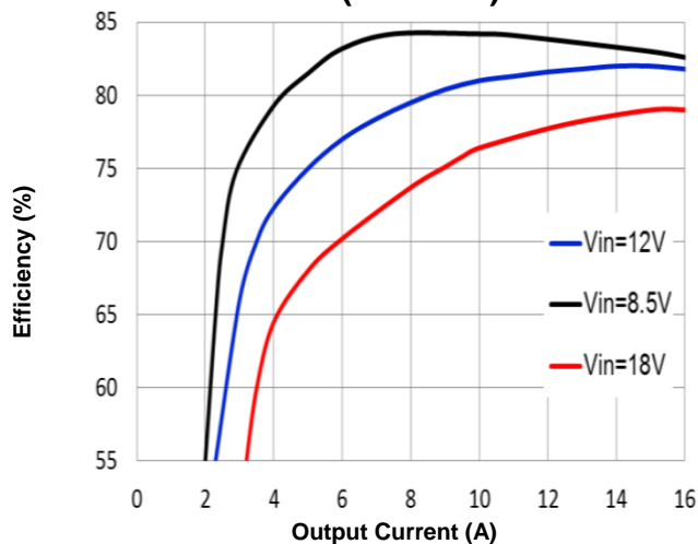
Figure 1a. Efficiency vs. Load Current (25°C)
