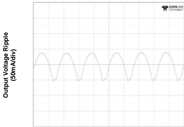
Figure 4c. Output Ripple Voltage (Vin=12V, full load)
