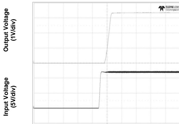
Figure 5d. Start-Up from Application of Input Voltage (Vin=12V, full load)
