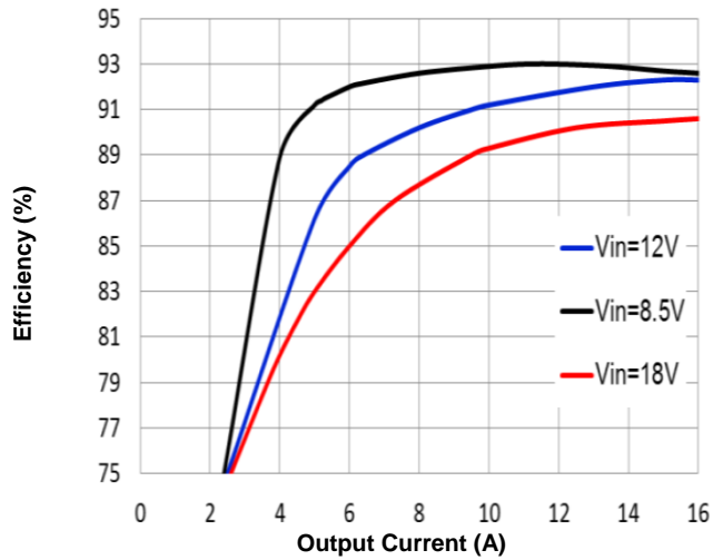
Figure 3a. Efficiency vs. Load Current (25°C)
