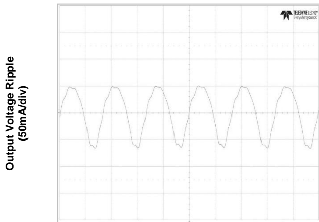
Figure 5c. Output Ripple Voltage (Vin=12V, full load)
