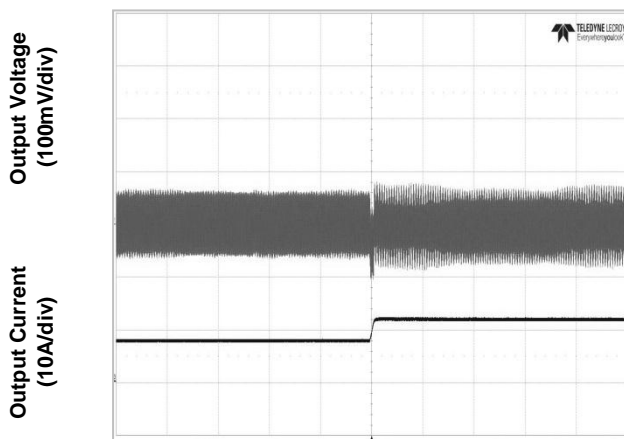
Figure 6e. Transient Load Response (typical Vin, load current steps from 50% to 75% at a slew rate 0.1A/µs)
