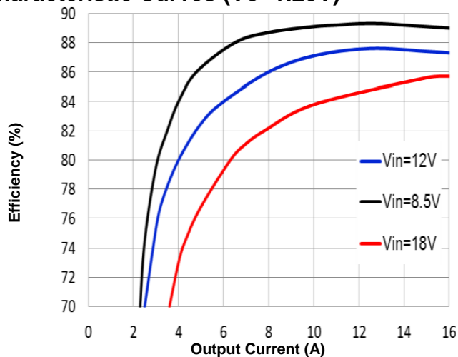
Figure 2a. Efficiency vs. Load Current (25°C)
