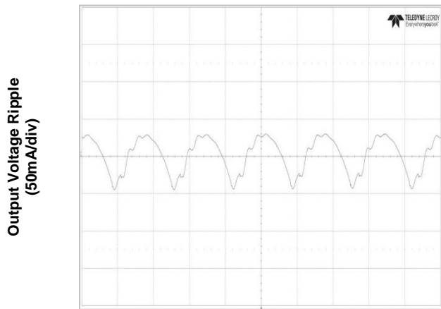
Figure 3c. Output Ripple Voltage (Vin=12V, full load)
