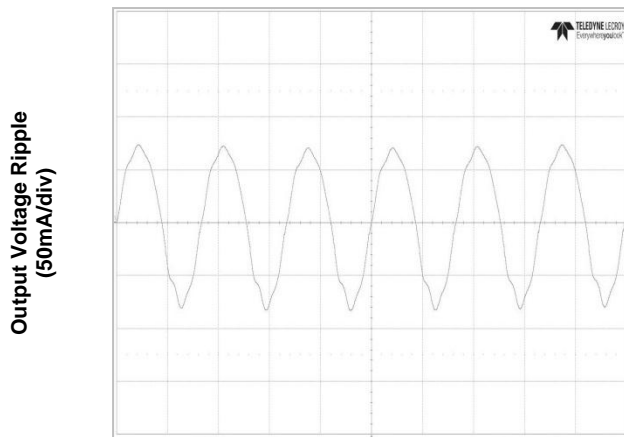
Figure 6c. Output Ripple Voltage (Vin=12V, full load)
