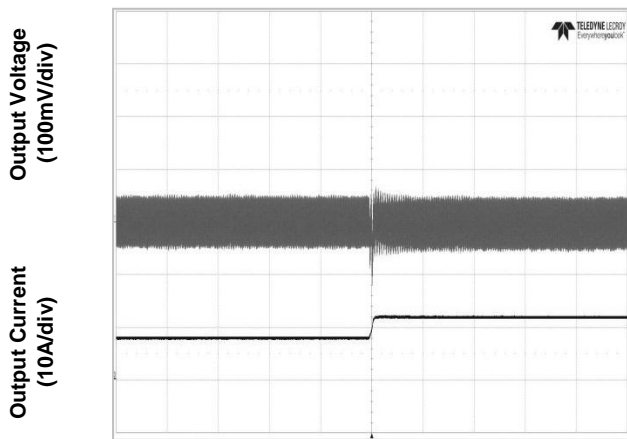
Figure 5e. Transient Load Response (typical Vin, load current steps from 50% to 75% at a slew rate 0.1A/µs)
