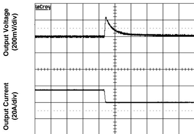
Time – t (200μs/div) Figure 8. Transient Load Response (typical V_{in} , load current steps from 75% to 50% at a slew rate 1A/μs)
