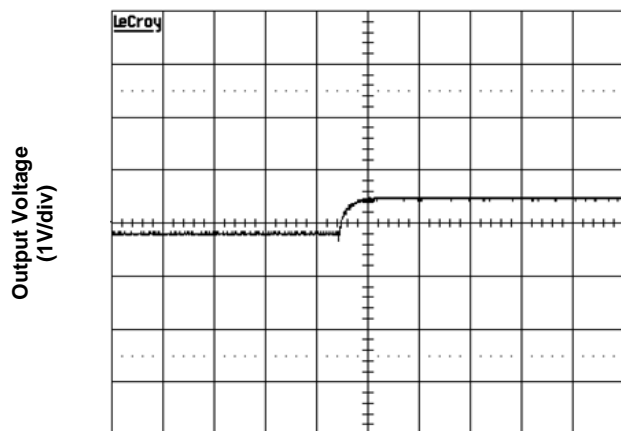
Time – t (10ms/div) Figure 6. Start-Up with Pre-bias ( V_{in}=12V , 2.5V/0A output, pre-bias voltage=1.8V)
