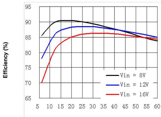
Figure 1c. Efficiency vs. Load Current (25°C, Vo=1.2V)
