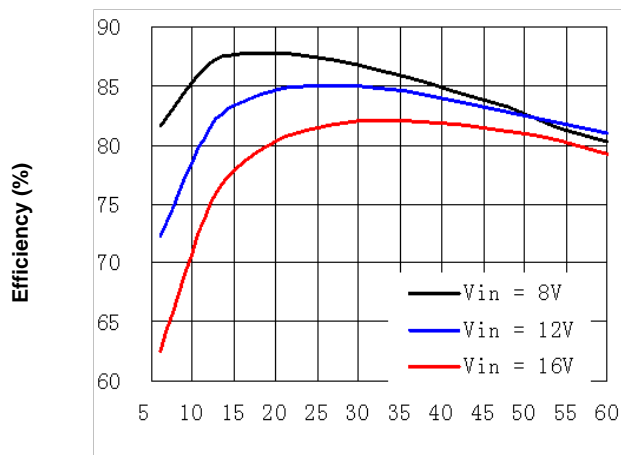
Figure 1a. Efficiency vs. Load Current (25°C, Vo=0.8V)
