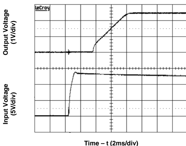
Figure 3. Output Ripple Voltage (2.5V/60A output)
