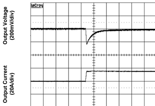
Time – t (200μs/div) Figure 9. Transient Load Response (typical V_{in} , load current steps from 50% to 75% at a slew rate 1A/μs)
