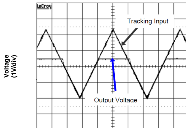
Time – t (10ms/div) Figure 7. Voltage Tracking/Sequencing (voltage tracking option, V_{in}=12V , V_o=2.5V , I_o=0A )
