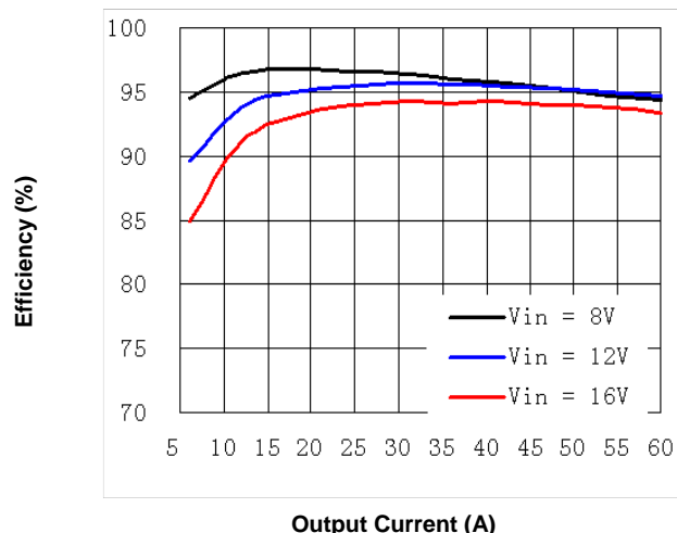
Figure 1h. Efficiency vs. Load Current (25°C, V_o=5V )
