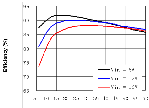
Figure 1d. Efficiency vs. Load Current (25°C, Vo=1.5V)
