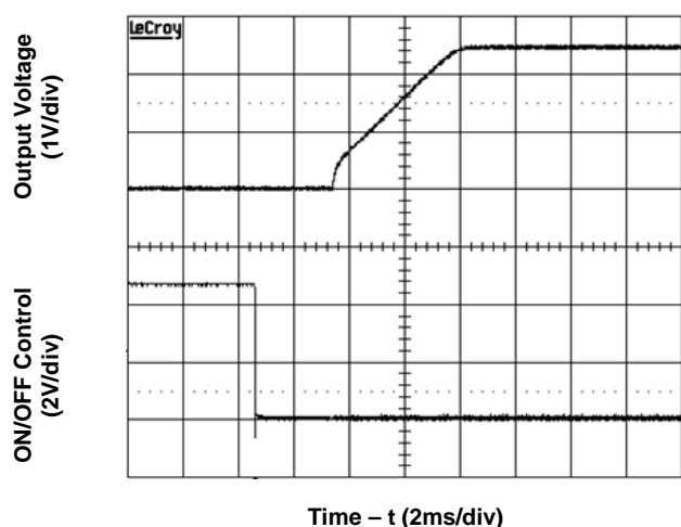
Figure 2. Input Characteristic (25°C, V_o=3.3V )
