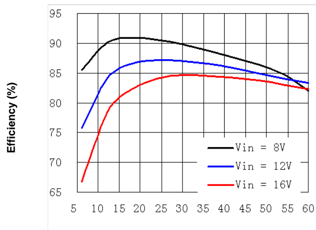
Figure 1b. Efficiency vs. Load Current (25°C, Vo=1.0V)
