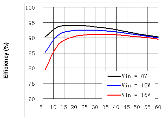
Figure 1f. Efficiency vs. Load Current (25°C, Vo=2.5V)
