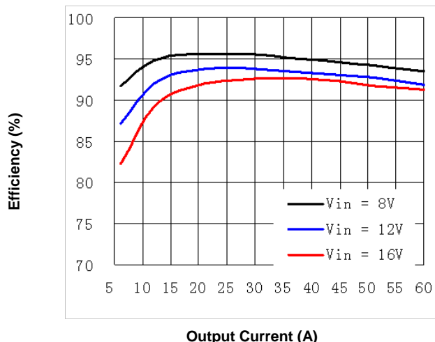
Figure 1g. Efficiency vs. Load Current (25°C, V_o=3.3V )
