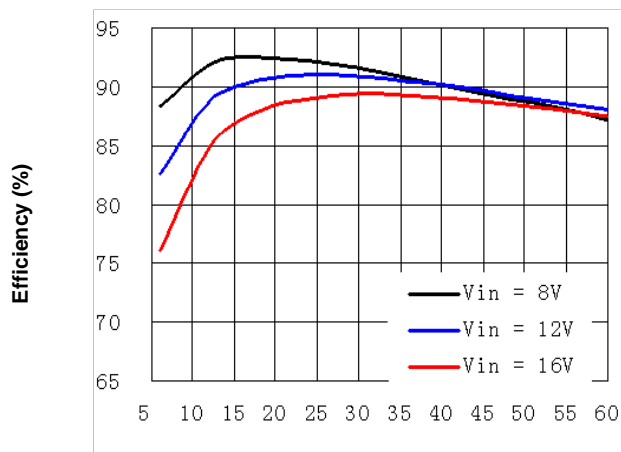
Figure 1e. Efficiency vs. Load Current (25°C, Vo=1.8V)
