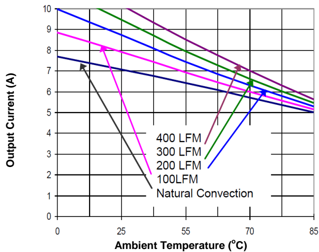
Figure 11a. Current Derating Curve (Vin=24V, Vo=5V, open frame)
