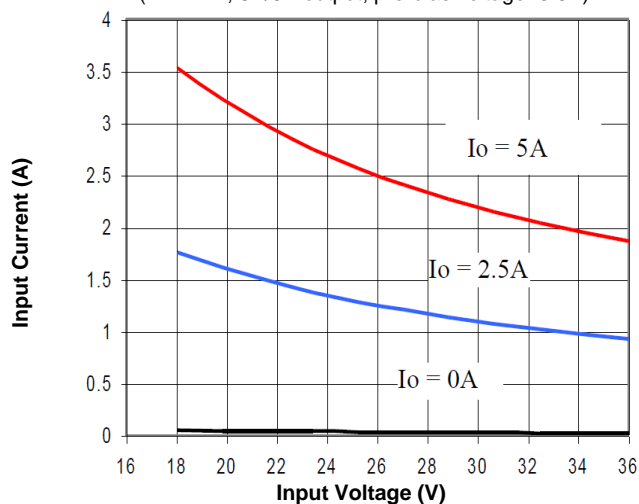
Figure 10. Input Characteristic ( V_o=12V )
