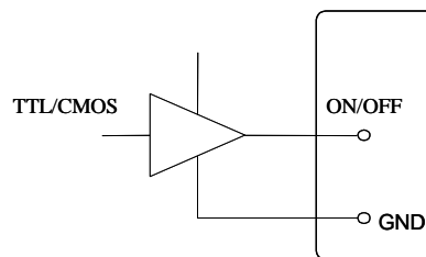
Figure 14. Direct Logic Drive
