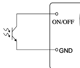
Figure 12. Opto Coupler Enable Circuit
