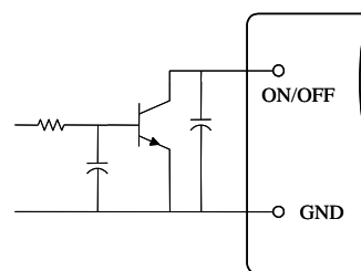
Figure 13. Open Collector Enable Circuit
