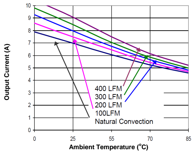
Figure 11b. Current Derating Curve (Vin=24V, Vo=12V, open frame)
