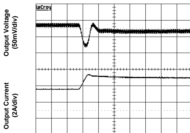
Figure 7. Transient Load Response (typical V_{in} , V_o=3.3V , load current steps from 3.75A to >5A at a slew rate 0.1A/ \mu s)
