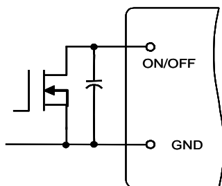
Figure 12. Circuit for Positive Logic Control
