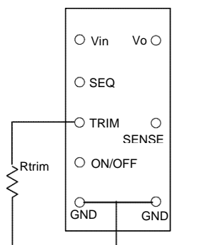
Figure 14. Circuit for Output Voltage Trim
