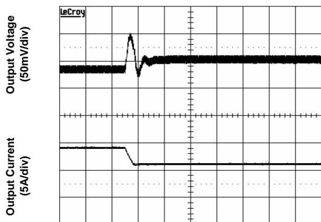
Figure 6. Transient Load Response ( V_{in}=5V , load current steps from 75% to 50% at a slew rate 0.1A/μs)
