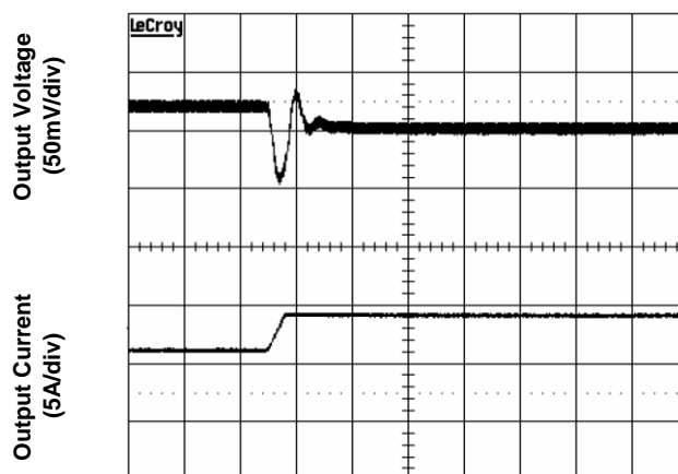
Figure 7. Transient Load Response ( V_{in}=5V , load current steps from 50% to 75% at a slew rate 0.1A/μs)
