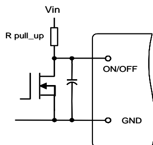
Figure 13. Circuit for Negative Logic Control
