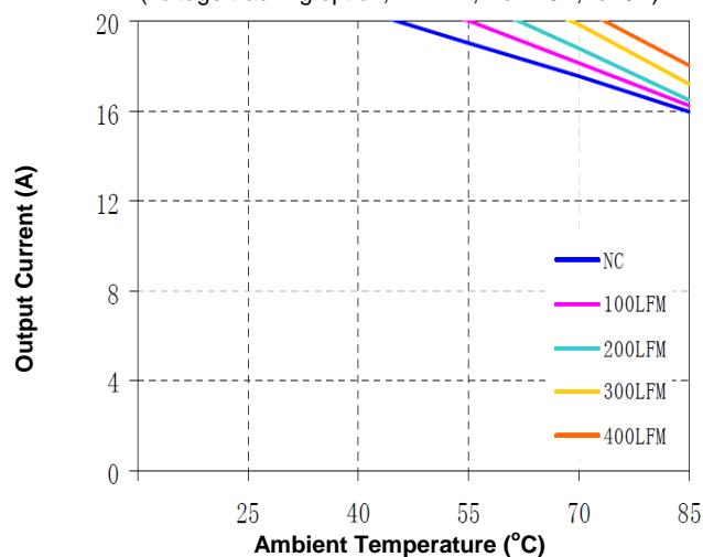
Figure 11b. Current Derating Curve (Vin=5V, Vo=1.2V, open frame)
