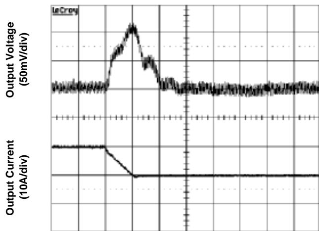
Figure 7. Transient Load Response (Vin=5V, load current steps from 100% to 50% at a slew rate 0.2A/μs)
