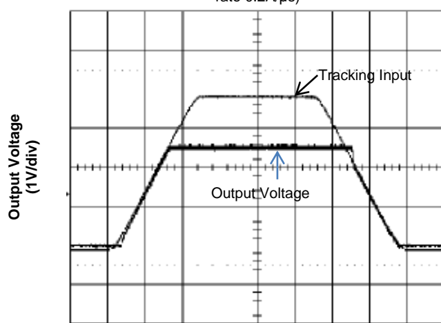
Figure 10. Voltage Tracking/Sequencing (voltage tracking option, Vin=4V, Vo=2.5V, Io=0A)
