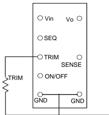
Figure 14. Circuit for Output Voltage Trim
