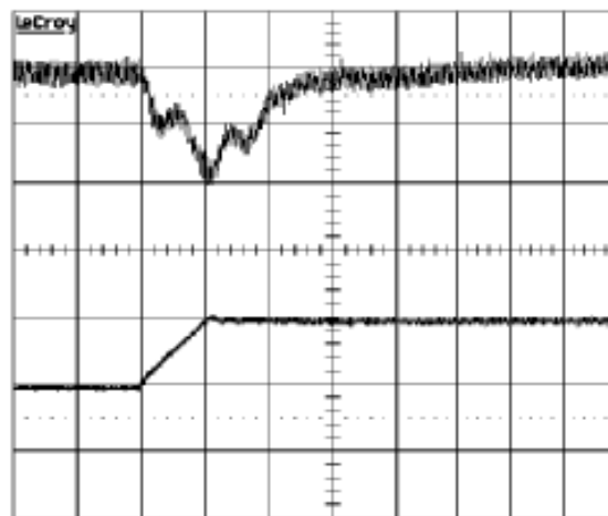
Figure 8. Transient Load Response (Vin=5V, load current steps from 50% to 100% at a slew rate 0.2A/μs)
