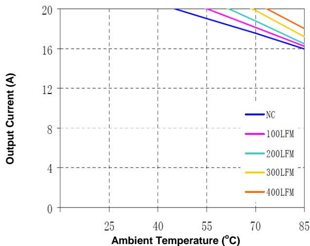
Figure 11a. Current Derating Curve (Vin=5V, Vo=1.0V, open frame)
