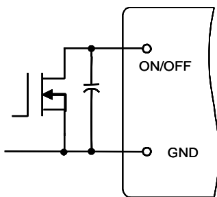
Figure 12. Circuit for Positive Logic Control
