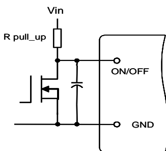
Figure 13. Circuit for Negative Logic Control
