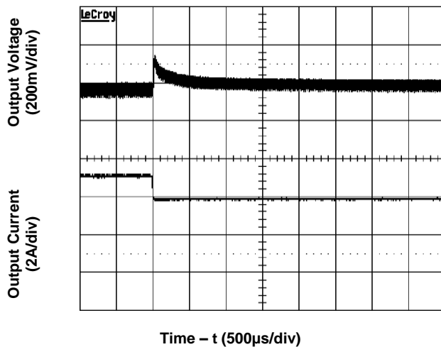
Figure 7. Transient Load Response
