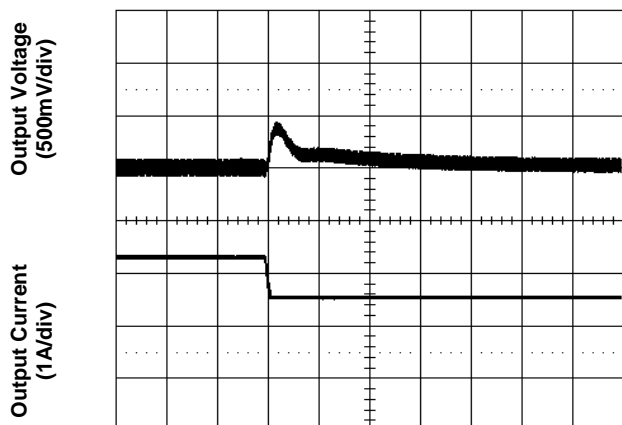
Figure 7. Transient Load Response
