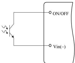
Figure 12. Opto Coupler Enable Circuit
