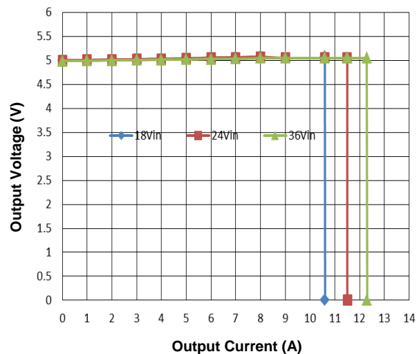
Figure 4. Output Characteristics
