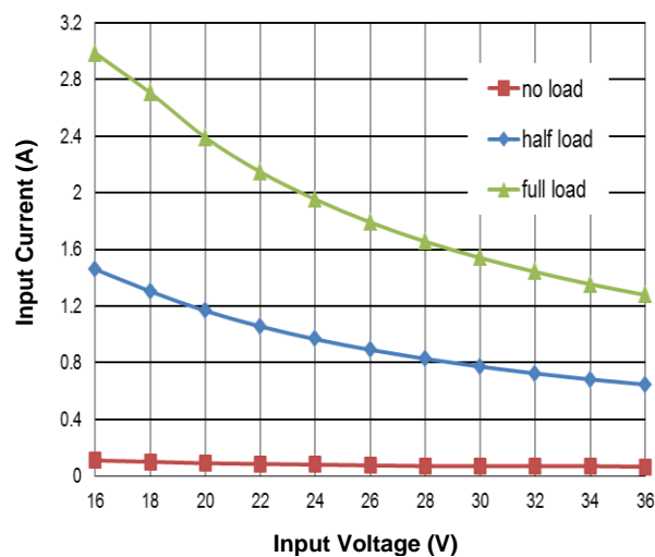
Figure 3. Input Characteristics
