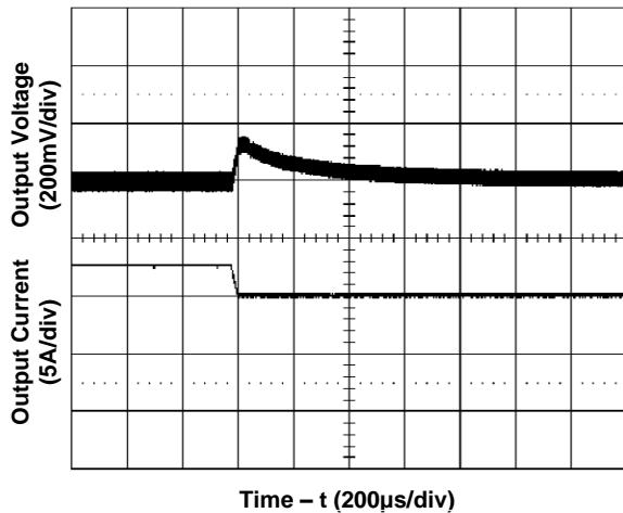
Figure 7. Transient Load Response
