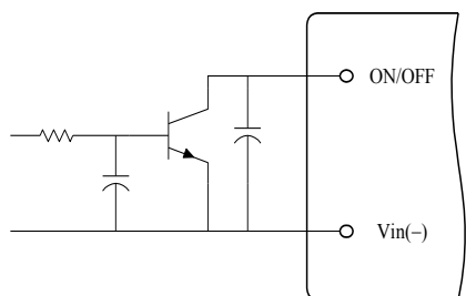
Figure 13. Open Collector Enable Circuit
