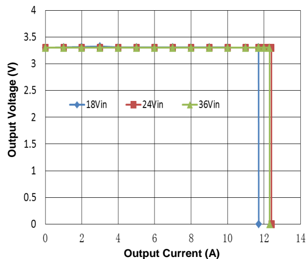
Figure 4. Output Characteristics (25°C)
