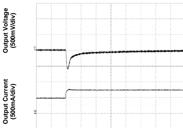
Time – t (500 \mu s/div) Figure 8. Transient Load Response (typical Vin, load current steps from 50% to 75% at a slew rate 0.1A/ \mu s)
