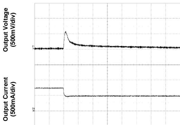
Time – t (500 \mu s/div) Figure 7. Transient Load Response (typical Vin, load current steps from 75% to 50% at a slew rate 0.1A/ \mu s)
