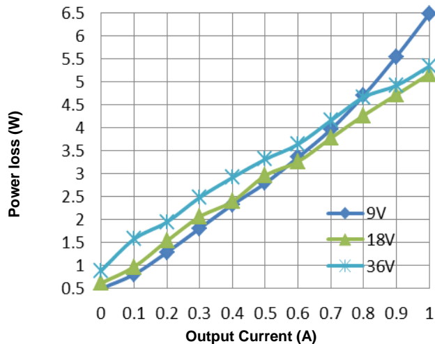
Figure 2. Power loss vs. Output Current (25°C)
