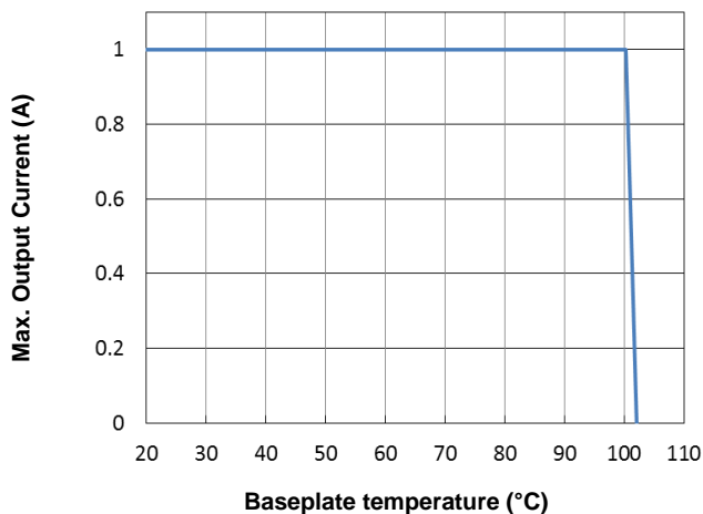
Figure 11. Current Derating Curve for Baseplate (typical Vin with baseplate; solder interface)
