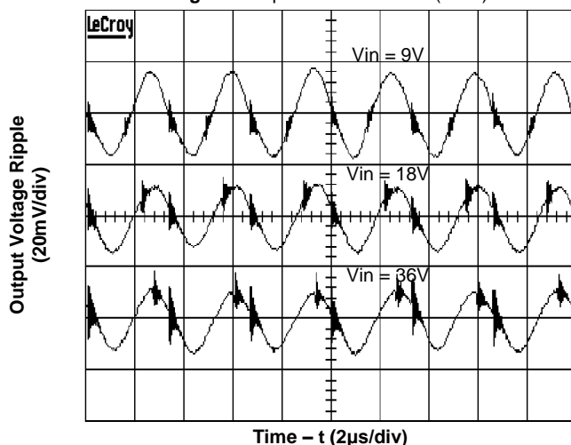
Figure 5. Output Voltage Ripple at Full Load (tested with 4x47µF ceramic output capacitors)
