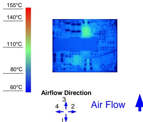
Figure 10. Thermal Image for Airflow Direction 3
