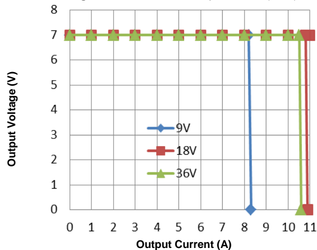
Figure 4. Output Characteristic
