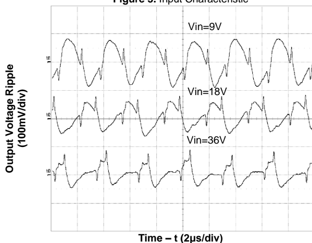
Figure 5. Output Ripple Voltage at Full Load (tested with 4x47μF ceramic output capacitors)
