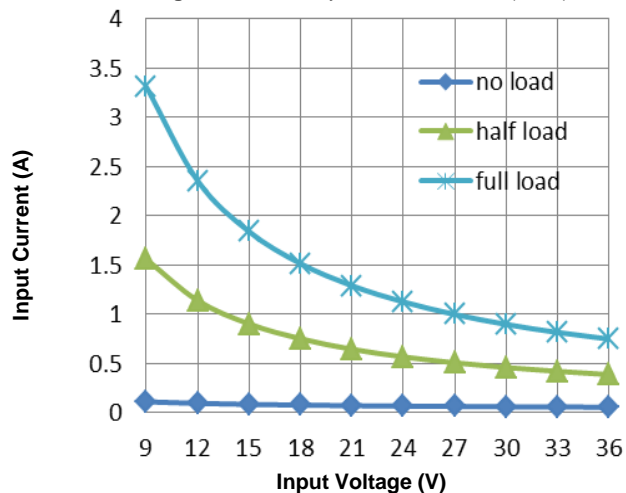
Figure 3. Input Characteristic
