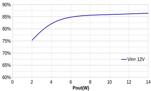
MGDD-21-E-E Typical Efficiency vs Output Power at T=25°C
