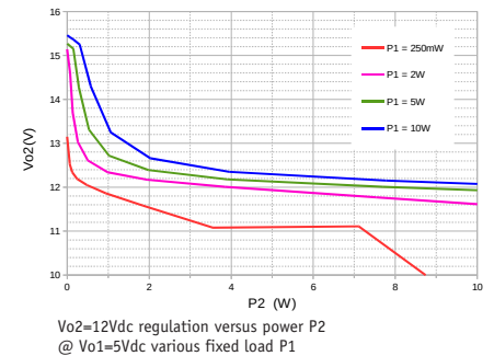
MGDD21-N-CE TYPICAL CROSS REGULATION @25°C
