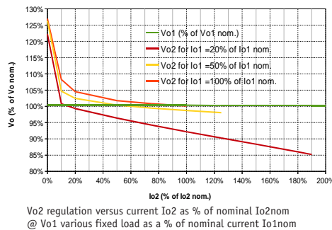
MGDD-21-N TYPICAL CROSS-REGULATION @ 25°C
