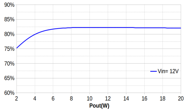
MGDD-21-E-C Typical Efficiency vs Output Power at T=25°C
