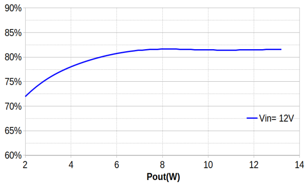
MGDD-21-E-B Typical Efficiency vs Output Power at T=25°C
