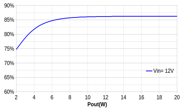
MGDD-21-E-F Typical Efficiency vs Output Power at T=25°C
