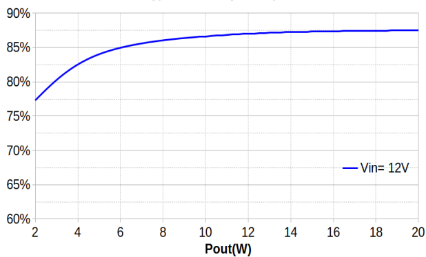
MGDD-21-E-I Typical Efficiency vs Output Power at T=25°C
