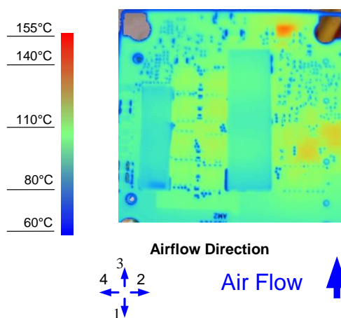
Figure 8. Thermal Image for Airflow Direction 3 (30A output, 55°C ambient, 200 LFM, typical Vin, open frame, socket interface)
