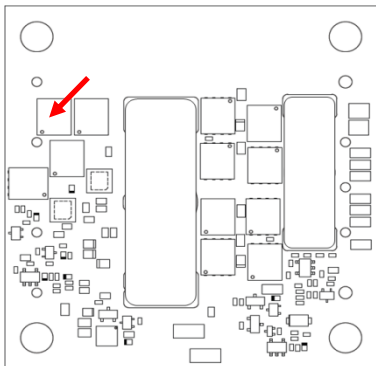
Figure 15. Temperature Monitoring Location
