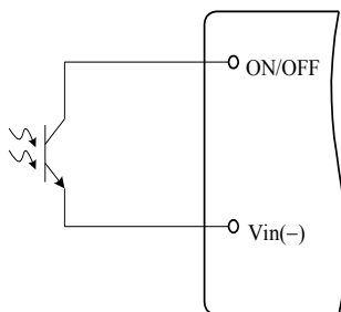
Figure 1. Opto Coupler Enable Circuit
