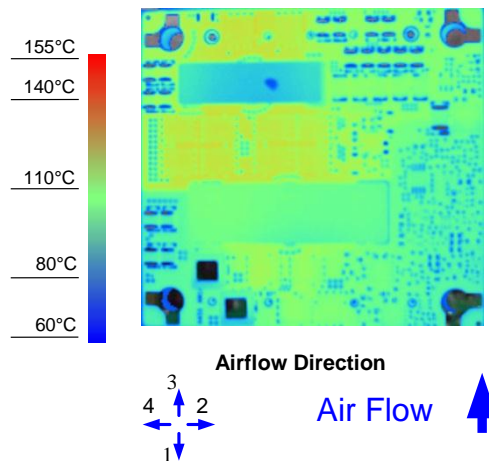
Figure 8. Thermal Image for Airflow Direction 3 (65A output, 55°C ambient, 200 LFM, typical Vin, open frame, unit soldered onto a fixture board)
