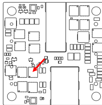
Figure 7. Temperature Monitoring Location
