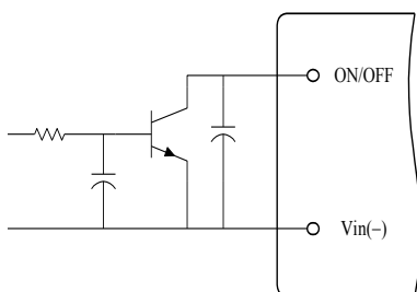
Figure 2. Open Collector Enable Circuit
