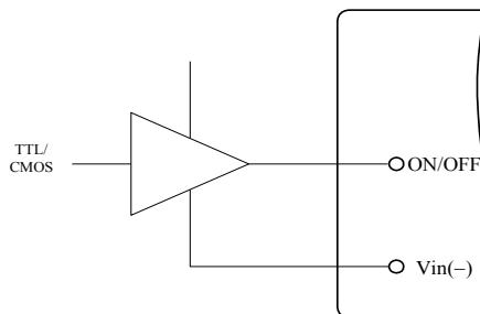
Figure 3. Direct Logic Drive
