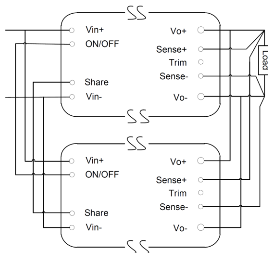
Figure 6. Circuit Configuration for Active Current Share
