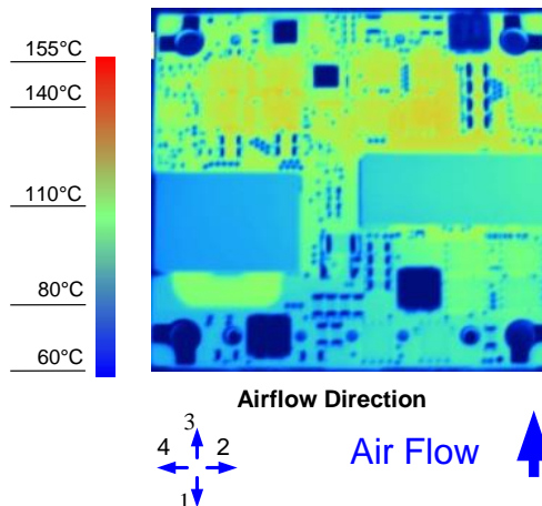
Figure 8. Thermal Image for Airflow Direction 3 (20A output, 55°C ambient, 200 LFM, typical Vin, open frame, unit soldered onto a fixture board)
