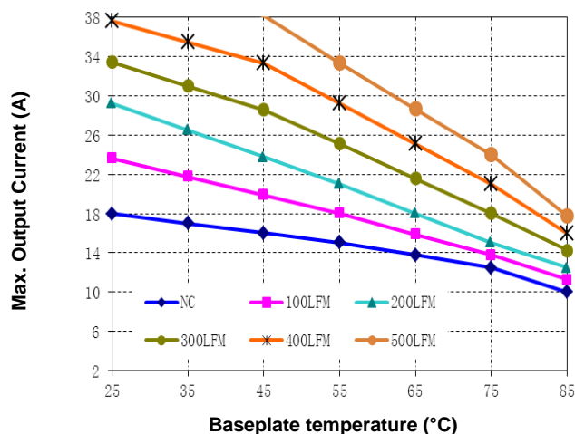
Figure 9. Current Derating Curve with Baseplate (typical Vin, soldered interface)
