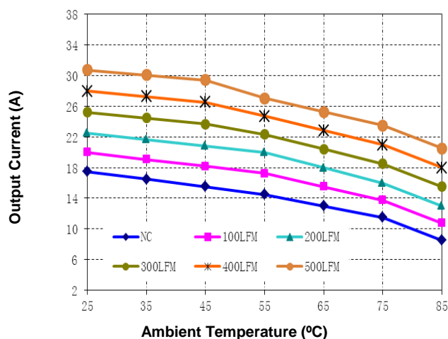
Figure 7. Current Derating Curve with Open Frame (Direction 3 (Ref. Figure 8); typical Vin, soldered interface)
