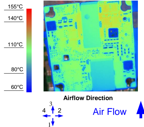
Figure 8. Thermal Image for Airflow Direction 3 (26A output, 55°C ambient, 200 LFM, typical Vin, open frame, unit soldered onto a fixture board)
