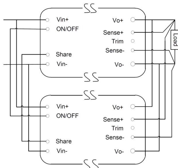
Figure 15. Circuit Configuration for Active Current Share
