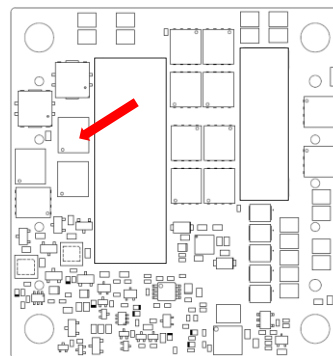
Figure 16. Temperature Monitoring Location
