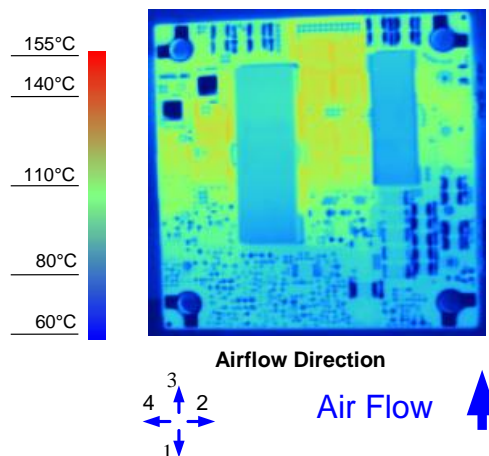
Figure 8. Thermal Image for Airflow Direction 3 (53A output, 55°C ambient, 200 LFM, typical Vin, open frame, unit soldered onto a fixture board)
