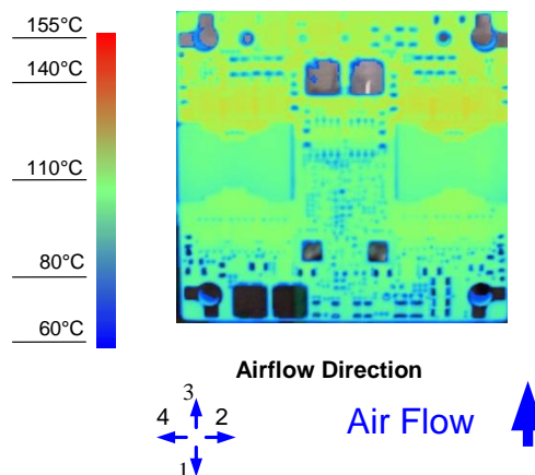
Figure 8. Thermal Image for Airflow Direction 3 (32A output, 55°C ambient, 200 LFM, typical Vin, open frame unit)
