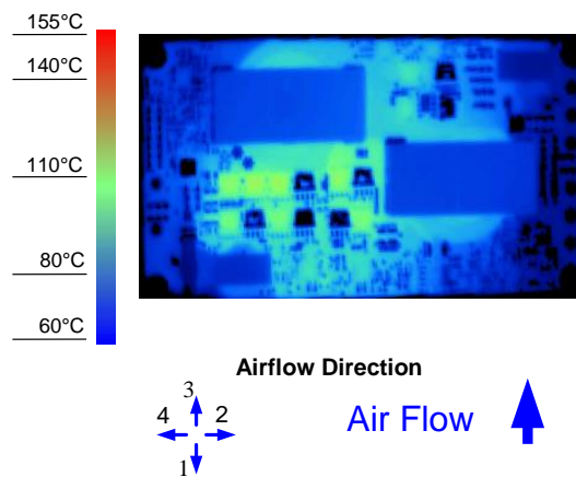
Figure 10. Thermal Image for Airflow Direction 3 (15.5A output, 55°C ambient, 200 LFM, typical Vin, open frame unit)
