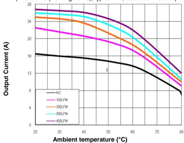
Figure 11. Current Derating Curve for Baseplate (Direction 3 (Ref. Figure 10); typical Vin, soldered interface)
