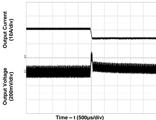
Figure 7. Transient Load Response (typical Vin, load current steps from 75% to 50% at a slew rate 0.1A/µs)
