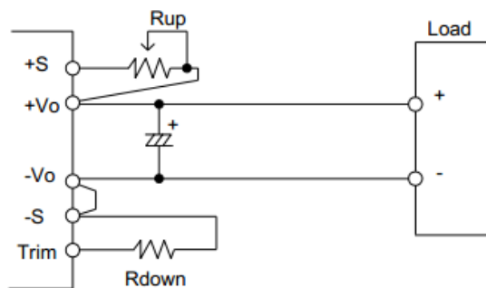
Figure 14. Trim Circuit
