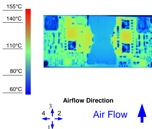
Figure 8. Thermal Image for Airflow Direction 3 (5A output, 55°C ambient, 200 LFM, typical Vin, open frame, socket interface)
