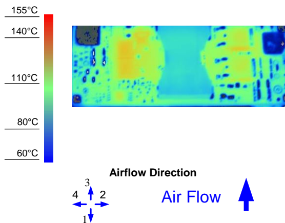
Figure 8. Thermal Image for Airflow Direction 3 (3A output, 55°C ambient, 200 LFM, typical Vin, open frame, socket interface)
