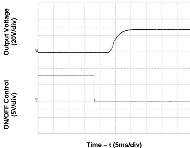
Figure 6. Start-Up from Enable Control (typical Vin, zero load)
