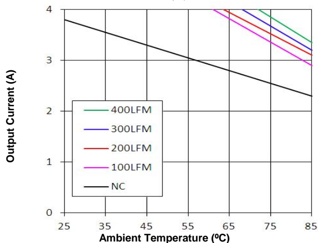
Figure 9. Current Derating Curve with Open Frame (Direction 3 (Ref. Figure 10); typical V_{in} )
