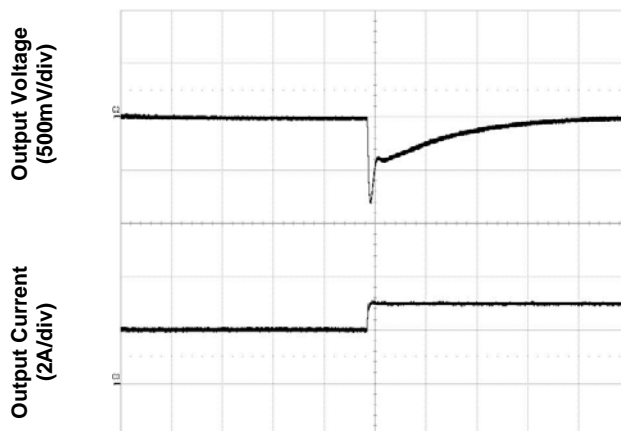
Figure 8. Transient Load Response (typical V_{in} , load current steps from 50% to 75% at a slew rate 0.1A/\mu s )
