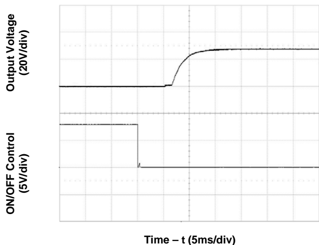
Figure 5. Start-Up from Enable Control (typical Vin, full load)
