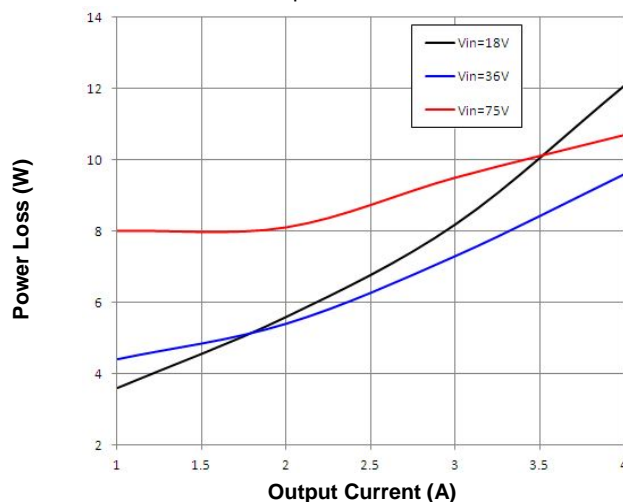
Figure 4. Power Loss vs. Load Current (25°C)
