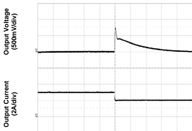
Figure 7. Transient Load Response (typical V_{in} , load current steps from 50% to 25% at a slew rate 0.1A/\mu s )
