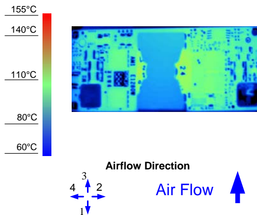
Figure 10. Thermal Image for Airflow Direction 3 (4A output, 55°C ambient, 200 LFM, typical V_{in} , open frame)
