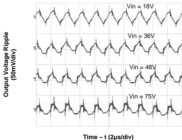
Figure 3. Output Ripple Voltage at Full Load
