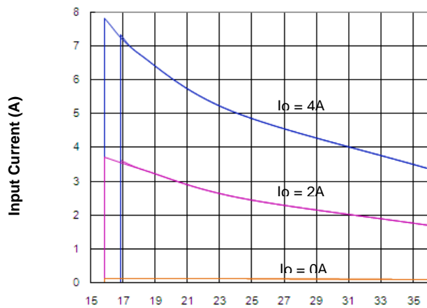
Figure 9. Input Characteristics (25°C)
