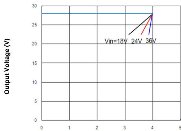
Figure 10. Output Characteristics (25°C)
