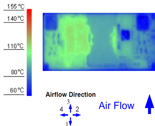
Figure 12. Thermal Image for Airflow Direction 3 (4A output, 55°C ambient, 200 LFM, V_{in} = 24V open frame unit)
