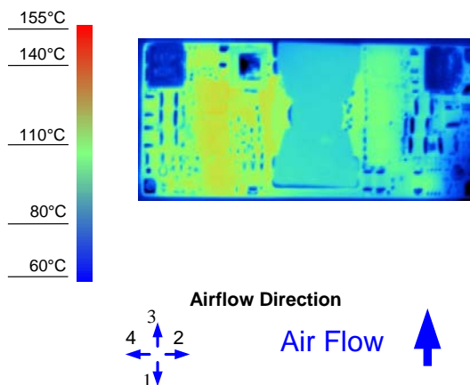
Figure 8. Thermal Image for Airflow Direction 3 (8A output, 55°C ambient, 200 LFM, typical Vin, open frame, unit soldered onto a fixture board)
