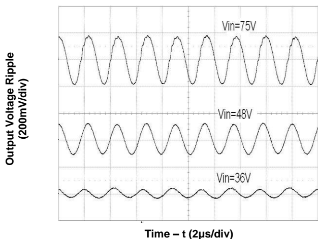
Figure 3. Output Ripple Voltage at Full Load
