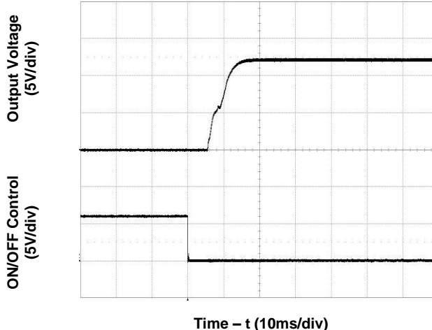
Figure 4. Start-Up from Enable Control
