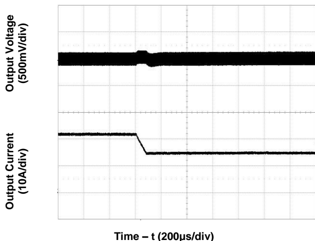
Figure 5. Transient Load Response (typical Vin, load current steps from 75% to 50% at a slew rate 0.1A/µs, 1,000µF external output capacitance)
