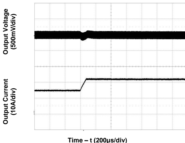
Figure 6. Transient Load Response (typical Vin, load current steps from 50% to 75% at a slew rate 0.1A/µs, 1,000µF external output capacitance)
