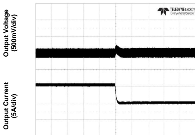
Figure 5. Transient Load Response (typical Vin, load current steps from 75% to 50% at a slow rate 0.1A/µs)
