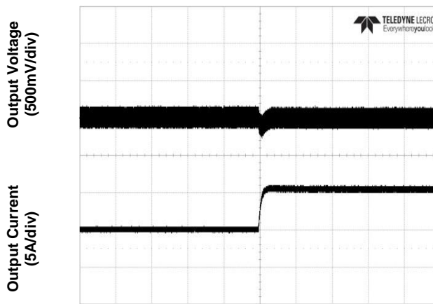
Figure 6. Transient Load Response (typical Vin, load current steps from 50% to 75% at a slow rate 0.1A/µs)
