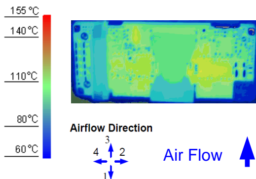
Figure 11. Thermal Image for Airflow Direction 3 (7A output, 55°C ambient, 200 LFM, typical Vin, unit soldered onto a fixture board)
