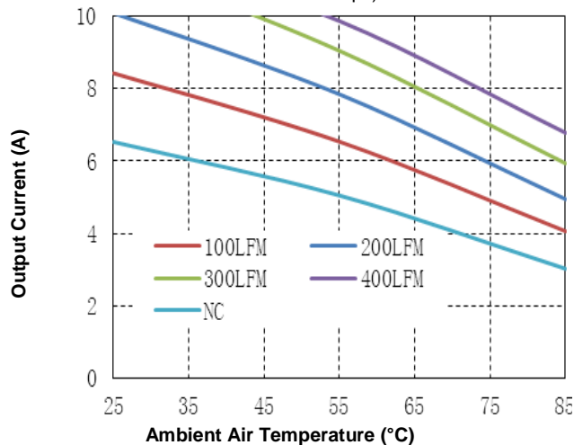
Figure 10. Current Derating Curve for Airflow Direction 3 (Ref. Fig. 11 for Airflow Direction; typical Vin, baseplate, unit soldered onto test fixture board)
