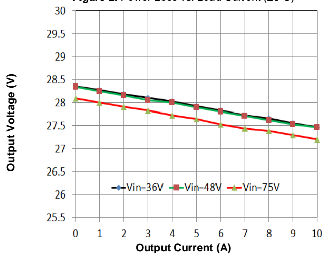
Figure 4. Output Droop Characteristic (parallel version)
