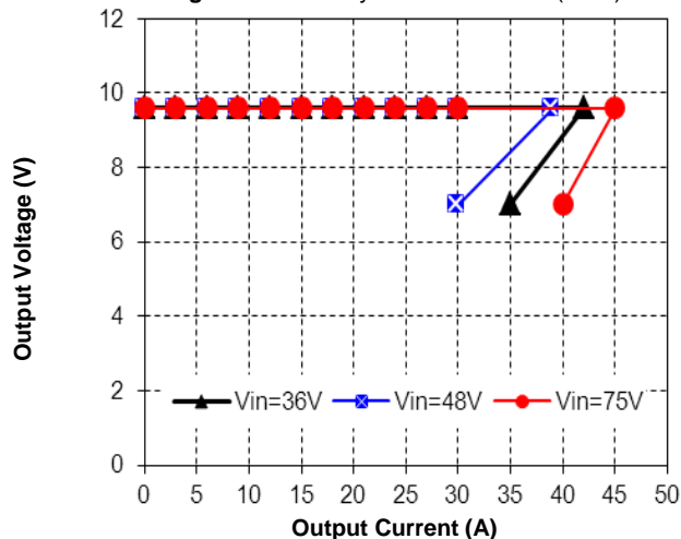
Figure 3. Output Characteristics (25°C) (Non-parallel version)
