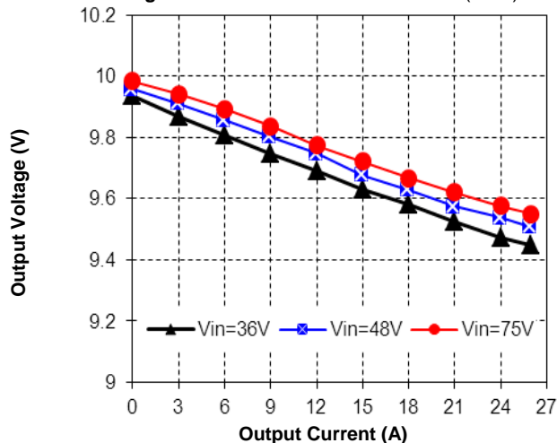
Figure 4. Output Characteristics (25°C) (Parallel version)
