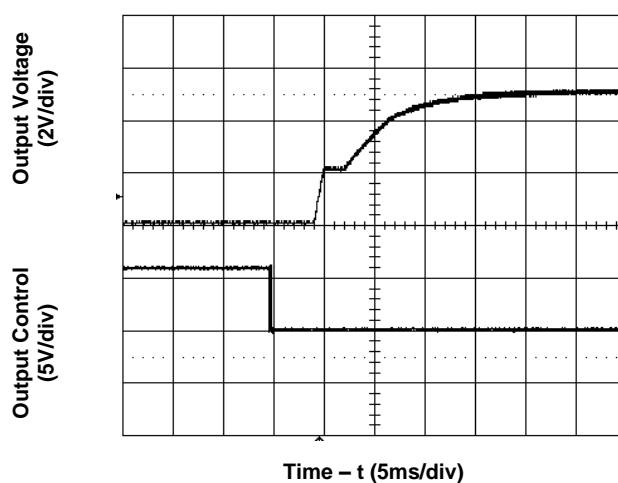
Figure 6. Start-Up from Enable Control
