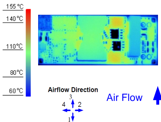
Figure 10. Thermal Image for Airflow Direction 3 (27.5A output, 55°C ambient, 200 LFM, typical Vin, open frame unit)
