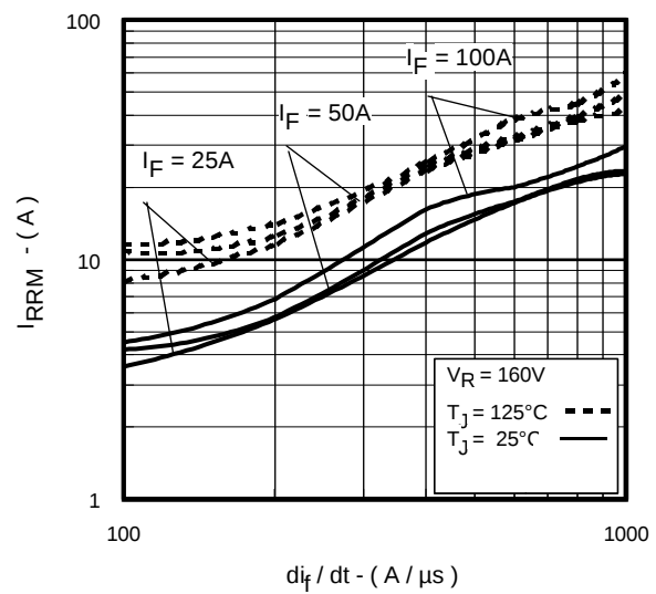
Fig. 6 - Typical Recovery Current Vs. di/dt (Per Leg)
